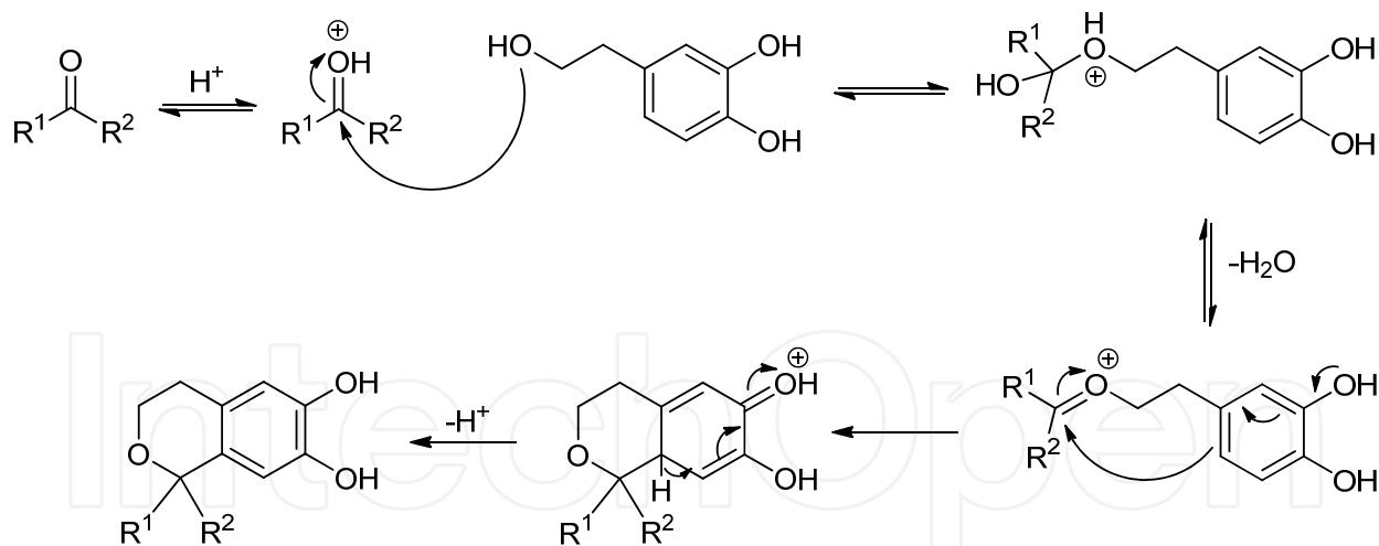
Scheme 9. Synthesis of hydroxytyrosol isochroman derivatives
