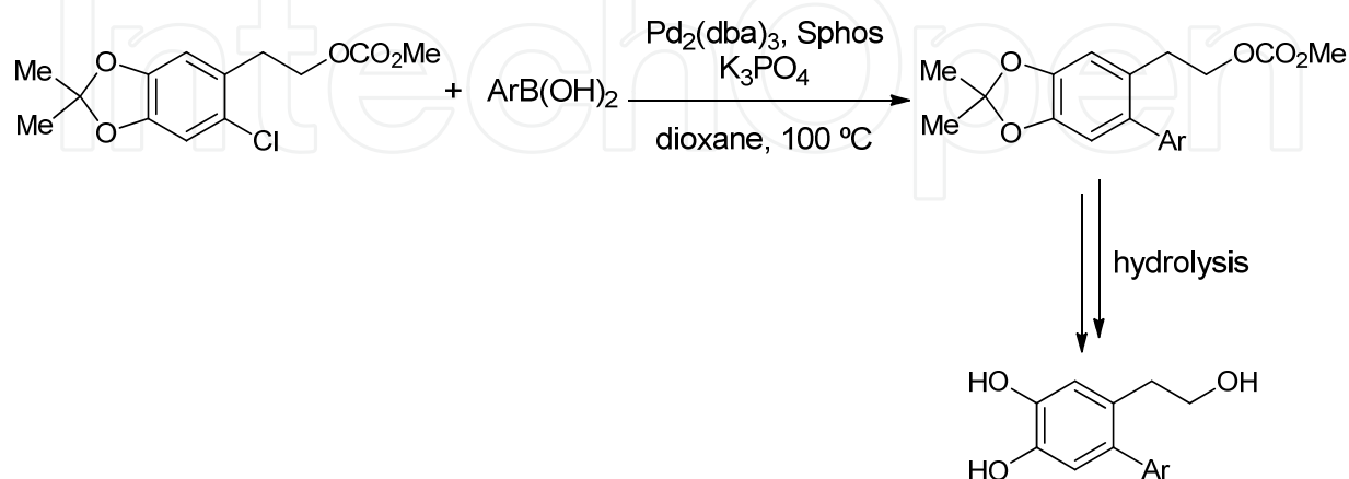
Scheme 11. Synthesis of 2-arylhydroxytyrosol derivatives
