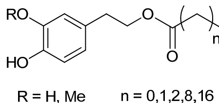
Fig. 3. Hydroxytyrosol lipophilic analogues
