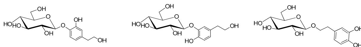
Fig. 5. The three isomers of hydroxytyrosol \beta -D-γλυχοπιρανοσιδεσ
