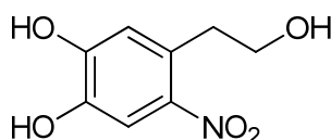
Fig. 2. 2-Nitrohydroxytyrosol formed by nitrosation of HT
