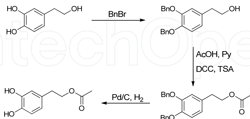
Scheme 2. Synthesis of hydroxytyrosyl acetate via benzylation of phenolic hydroxyls
