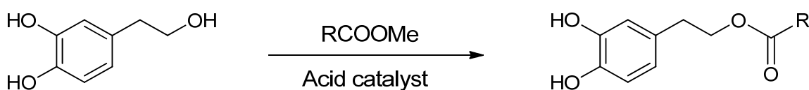
Scheme 4. General procedure of acid-catalyzed transesterification
