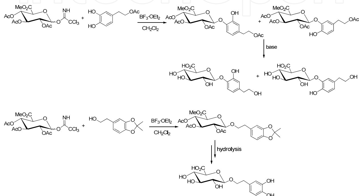
Scheme 10. Synthesis of hydroxytyrosol glucuronides
