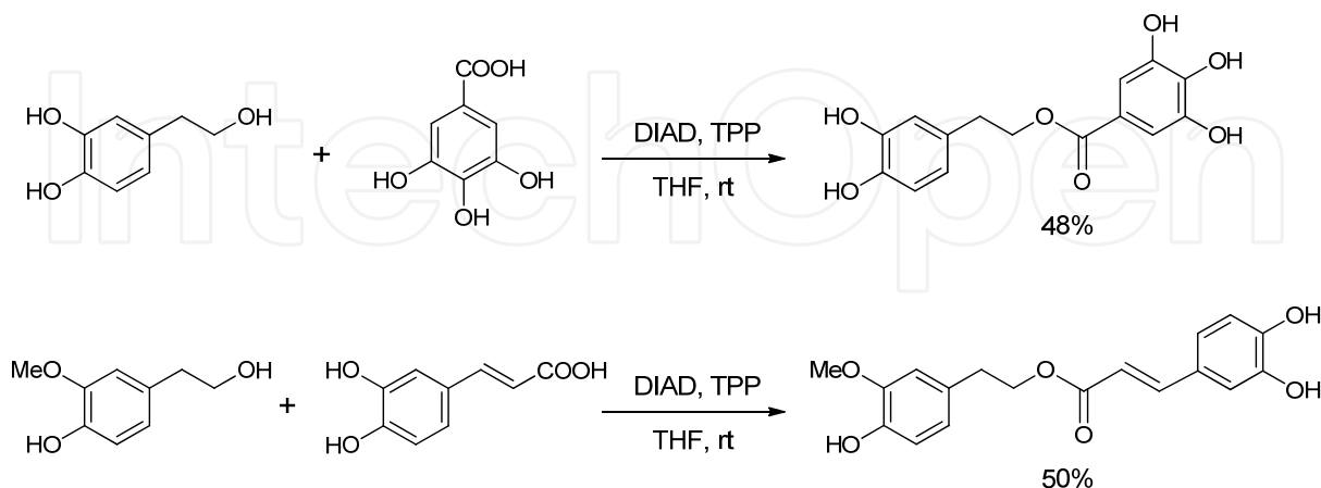
Scheme 6. Mitsunobu esterification of hydroxytyrosol and vanillyl alcohol
