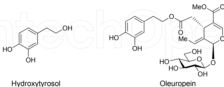
Fig. 1. Structures of hydroxytyrosol and oleuropein
