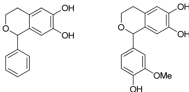
Fig. 4. Isochromans naturally present in olive oil
