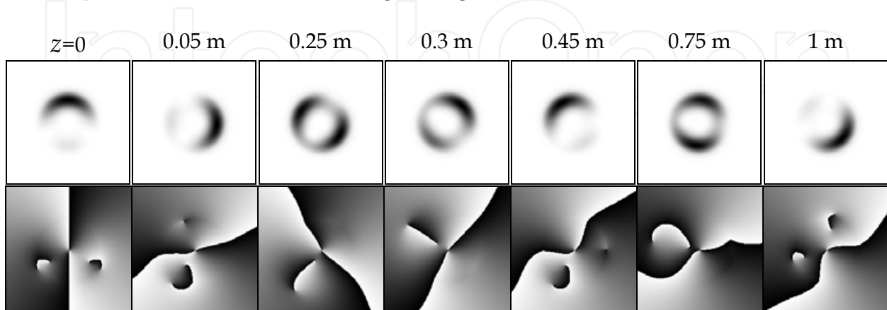
Fig. 7. In propagation, the superposition of (p,q) modes: (2,1)+(3,1)+(4,1) , is nearly self-reproduced at distance z_L=1 \text{ m} (intensity and phase distributions are depicted at various distances z ).
