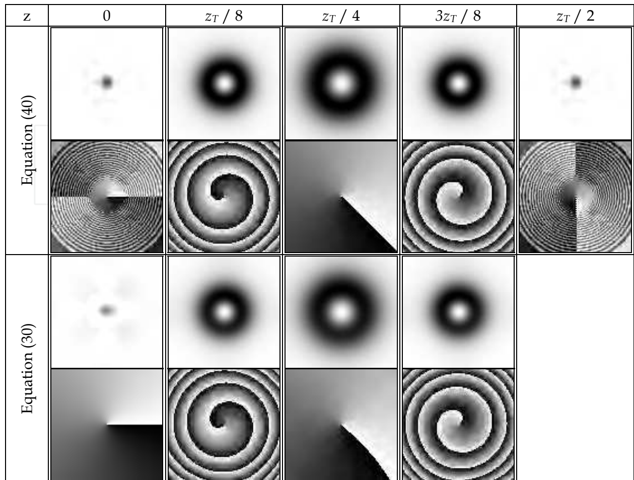
Fig. 20. Propagation Gaussian optical vortex with \mu = 1 ( \sigma = \sigma_0/2 ).
