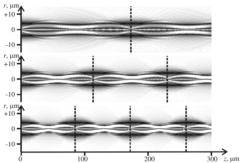
Fig. 21. Propagation of Gaussian optical vortex in parabolic waveguide for various values of parameter \alpha : \alpha = 17.88 \text{ mm}^{-1} (top part), \alpha = 26.82 \text{ mm}^{-1} (central part) and \alpha = 35.76 \text{ mm}^{-1} (bottom part). Dashed lines mean periods of diffraction patterns (i.e. planes z = p\pi / \alpha , where p are integer numbers).
