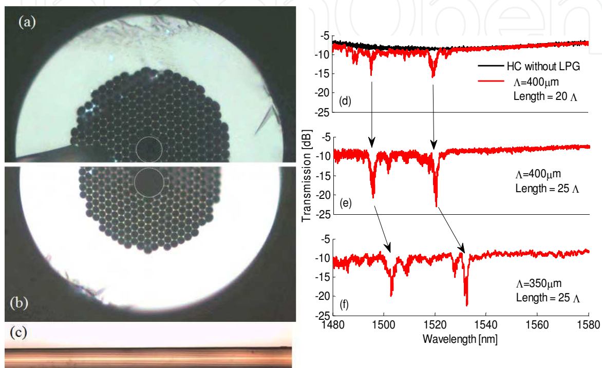
Fig. 15. Optical microscopy images of HC-PCF cross-section (a) before and (b) after EAD procedure; (c) Optical microscopy image of LPG with \Lambda=400\mu\text{m} (20 periods); transmitted spectra of LPG in HC-PCF with (d) 20 periods and \Lambda=400\mu\text{m} , (e) 25 periods and \Lambda=400\mu\text{m} , and (f) 25 periods and \Lambda=350\mu\text{m} . (Iadicicco et al., 2011).
