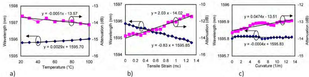
Fig. 17. Measured resonant wavelength and peak transmitted attenuation of the LPG in HC-PCF as functions of a) temperature, b) tensile strain and c) curvature. Reprinted from (Y. Wang et al., 2008) with permission of Optical Society of America.
