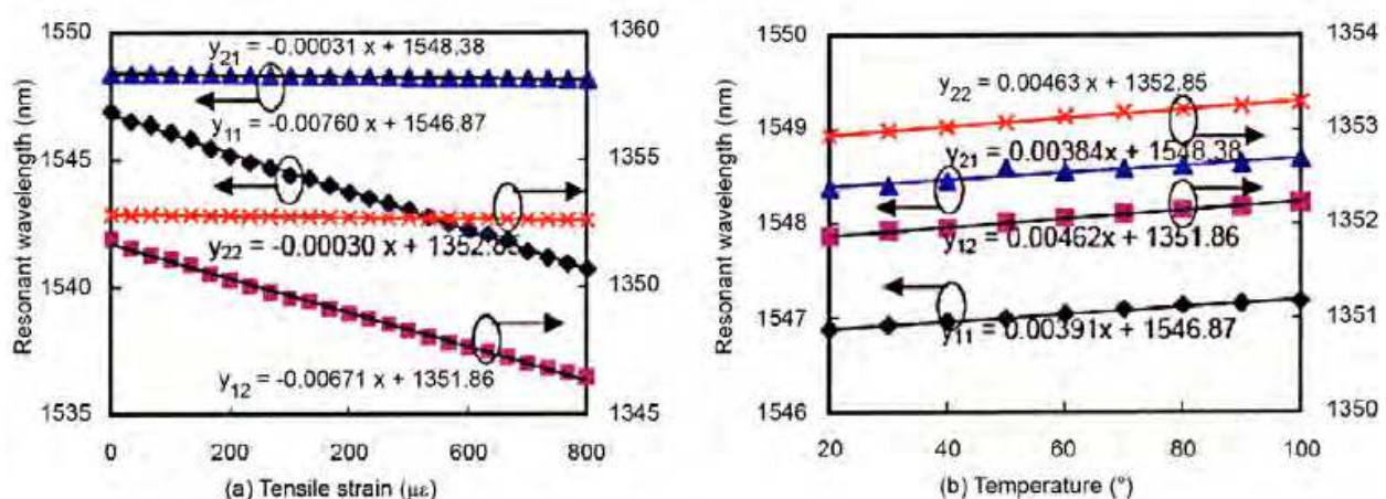
Fig. 16. Resonant wavelength of LPFG via (a) the tensile strain and (b) the temperature: ◆ and ■ refer to LPG with period grooves and ▲ and X refer to LPG without period grooves. Reprinted from (Y. Wang et al. 2006) with permission of Optical Society of America.
