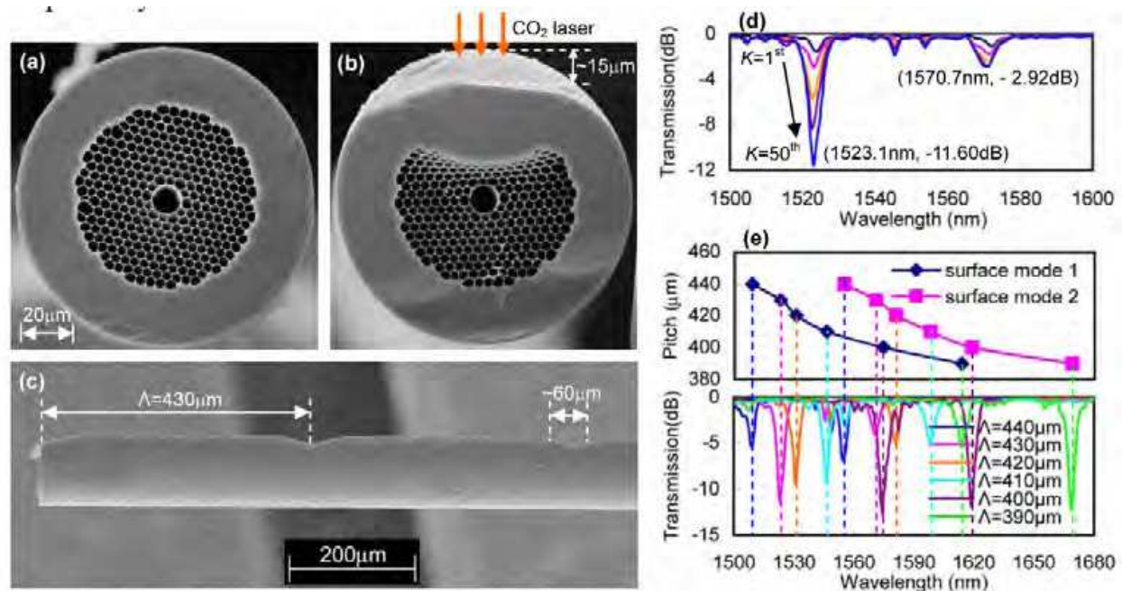
Fig. 14. Scanning electron micrographs of HC-PCF cross-sections (a) before and (b) after \text{CO}_2 laser irradiation; (c) LPG on HC-PCF with 50 scanning cycles; (d) Evolution of the transmitted spectrum of LPG with 40 periods and a grating pitch of 430\mu\text{m} with increasing number of scanning cycles; (e) Variation of LPFG resonant wavelengths with grating pitch. Reprinted from (Y. Wang et al., 2008) with permission of Optical Society of America.
