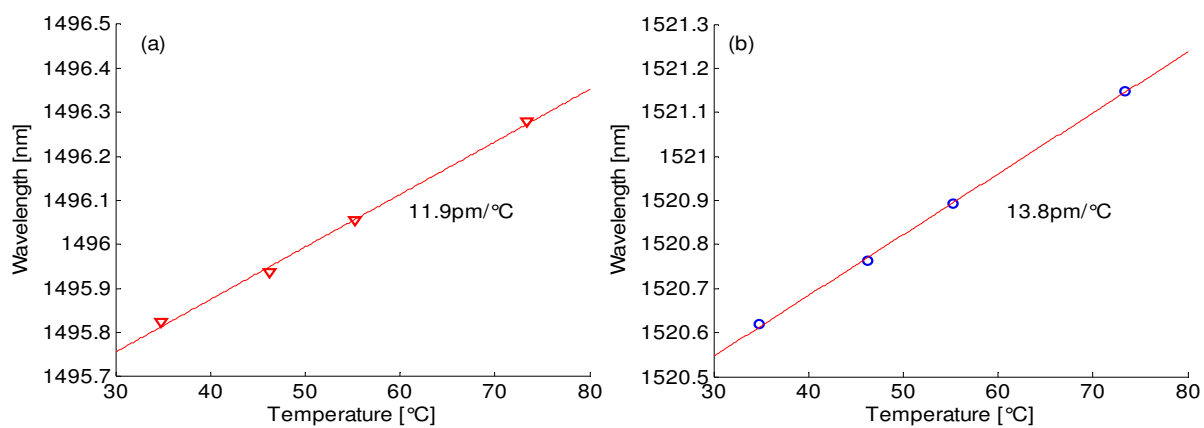
Fig. 18. Measured resonant wavelengths of the LPG in HC-PCF achieved by EAD as functions of temperature for left (a) and right (b) band.
