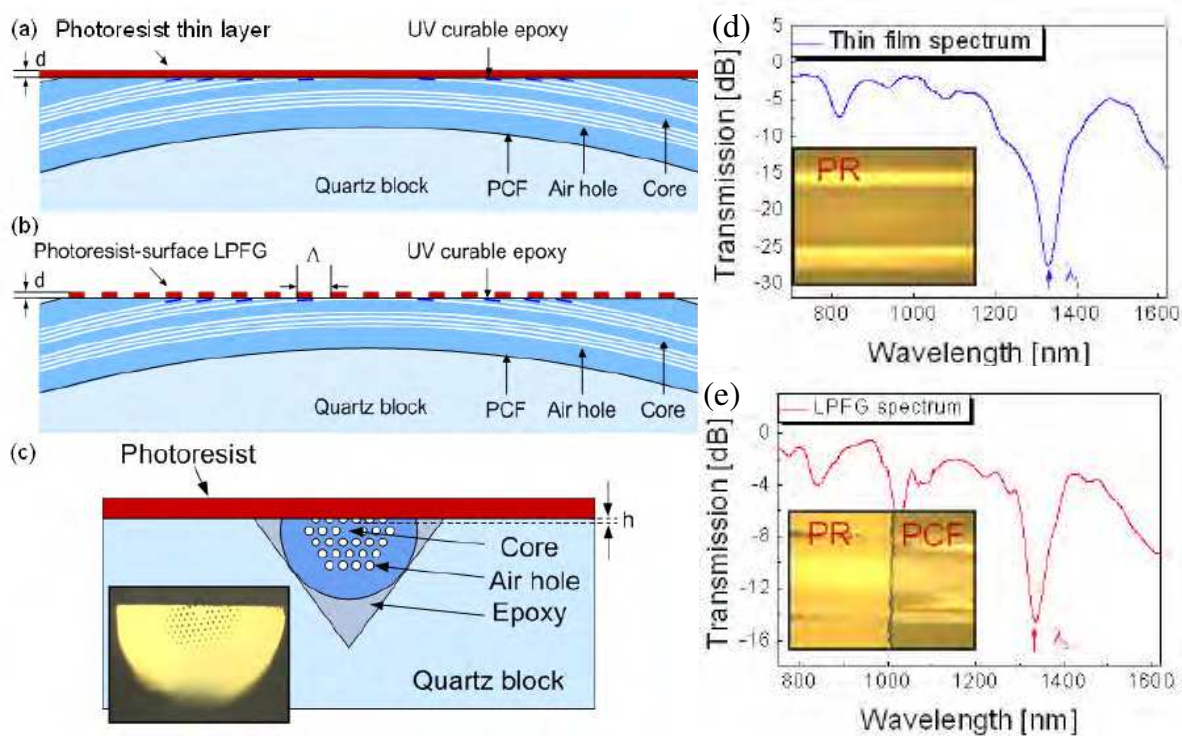
Fig. 7. Schematic diagram (not in scale) of (a) the uniform thin layer along the D-shaped PCF, (b) the PCF-based surface LPFG, and (c) the cross section of the D-shaped PCF with the photoresist overlay; transmission spectrum of (d) the PCF-based thin layer and (e) the PCF-based surface LPFG. Reproduced with permission from (H. Kim et al., 2010).
