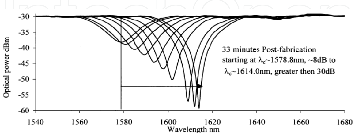
Fig. 2. Post-fabrication spectral evolution of an attenuation band from a D-fiber based LPG (period of 400\ \mu\text{m} ). Reproduced with permission from (Allsop et al., 2004).
