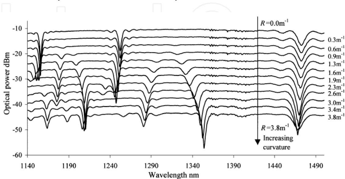
Fig. 9. Evolution of the transmission spectrum of a D-fiber based LPG (period of 380 \mu\text{m} ) subjected to bending, showing the appearance of bend induced stop-bands. (Reproduced with permission from (Allsop et al., 2004)).
