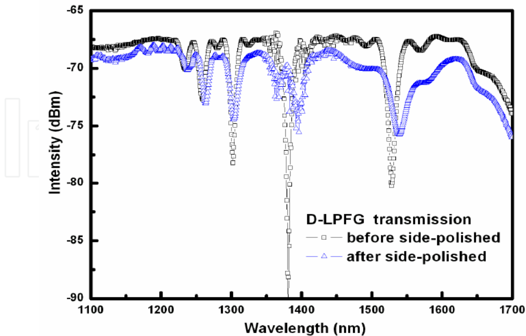
Fig. 4. Transmission spectra before and after side-polishing of the LPG. Reproduced with permission from (Tien et al., 2009a).
