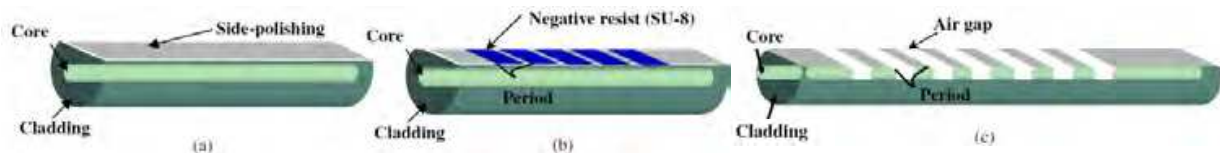
Fig. 5. Schematic diagram of the fabrication steps for the realization of AG-LPGs (not in scale). Reproduced with permission from (Fu et al., 2011).
