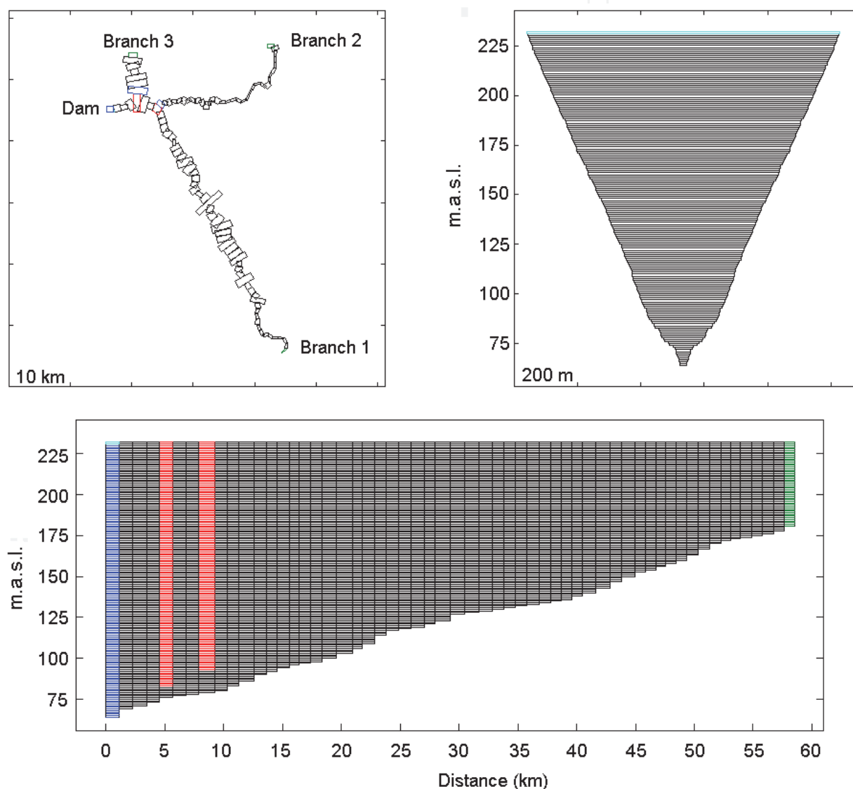
Fig. 6. Bathymetry grid of Santiago river or Branch 1. This graphic illustrates the location of the aforementioned branch at the top left side and shows the cross-section of its deepest part at the top right side. The cross-section is then identified with a blue color in the horizontal profile of this branch at the bottom of this figure, where the red grids represent the connection between Branch 2 and 3 with Branch 1 and green grids correspond to the shallowest section of Santiago river.
