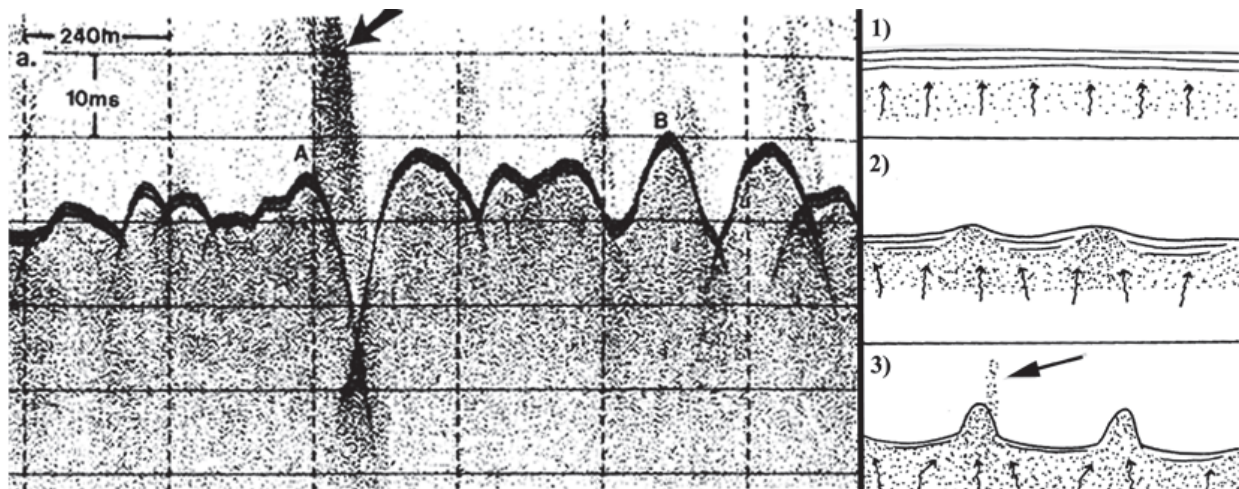
Fig. 14. Seepage and evidence of deforming clay at the Onyx field, off Mid-Norway (Based on Hovland 1990a and 2008). The sketches to the right, numbered 1 - 3 indicates a novel development model suggested by Hovland (1990a). See text for further description.
