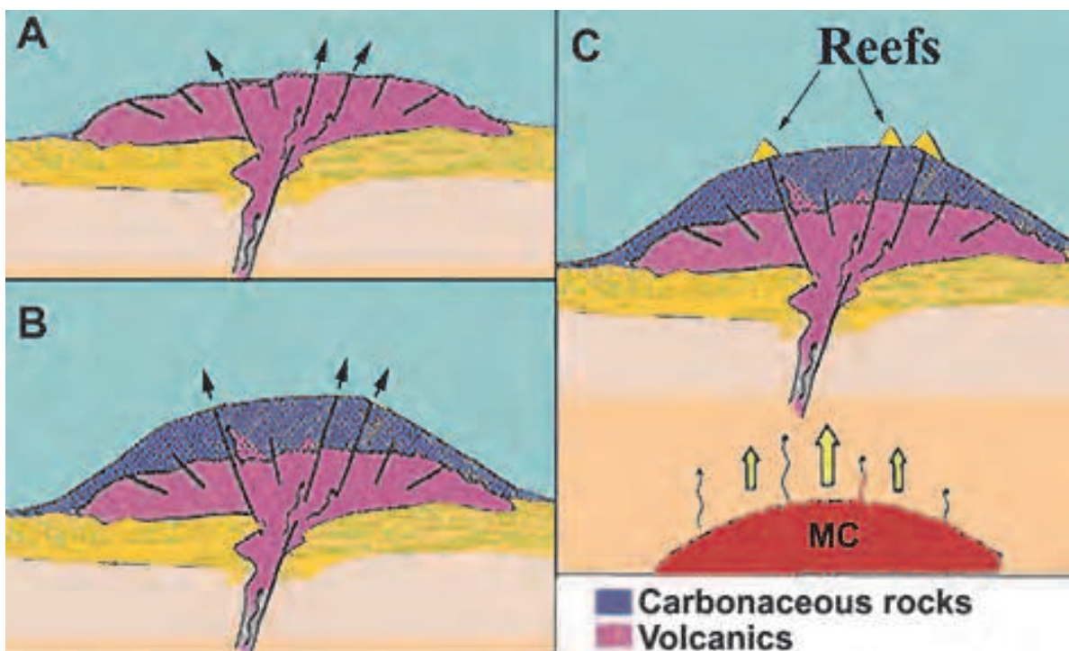
Fig. 3. Conceptual cartoon (based on Belka, 1998) indicating in chronological order (A, B, C) how volcanic outflow onto the seafloor may have stimulated the growth of the carbonate mounds (yellow cones, denoted "Reefs") of Sahara. "MC" = magma chamber.
