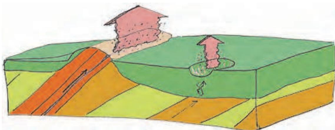
Fig. 1. Seepage of fluids (liquids and gas) though the seafloor may occur through positive seafloor relief (left arrow) or it may induce negative relief features in the seafloor (right arrow).
