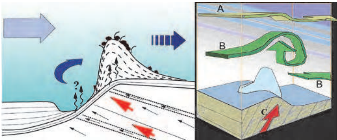
Fig. 17. The DWCR Hydraulic theory is illustrated in these two sketches. The concept is based on the idea that nutrients are brought up to the seafloor surface through seepage (red arrows). The arrow A represents the general prevailing current, B is the turbulent near-bottom current, and C, fluid flow (seepage) from below (Based on Hovland, 2008).
