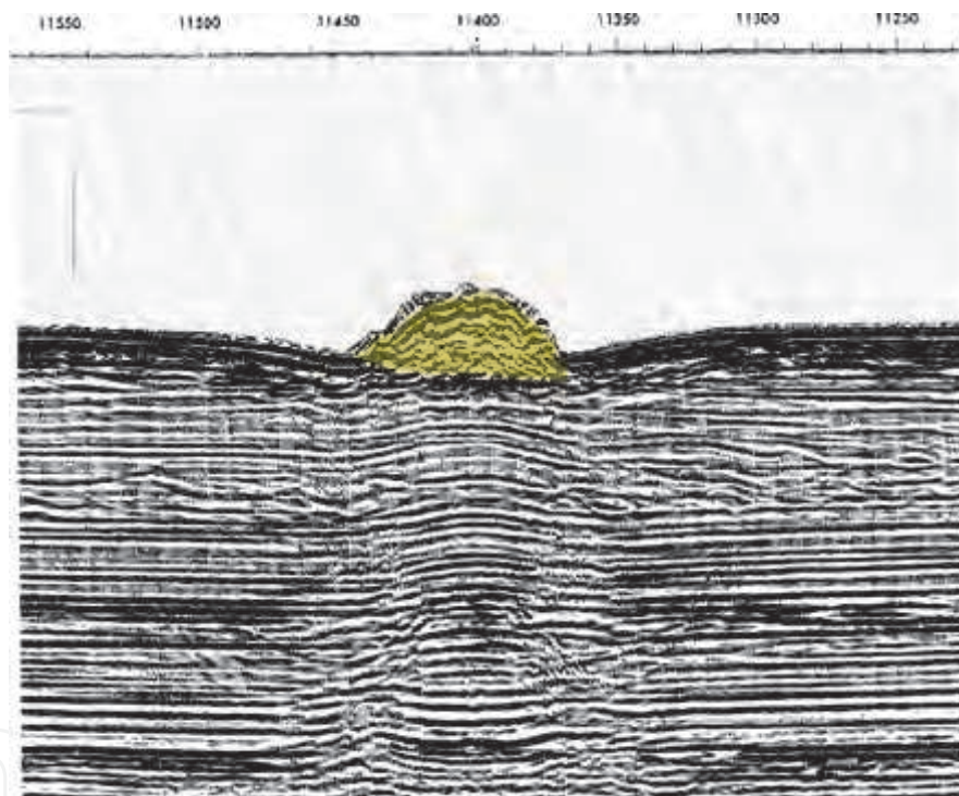
Fig. 22. A 2D reflection seismic image of a live, giant carbonate mound (yellow) off SW-Ireland (Hovland et al., 1994b). The height of the carbonate mound is about 100 m and its length at base is about 1 km. The water depth is about 800 m (see also Hovland, 2008).
