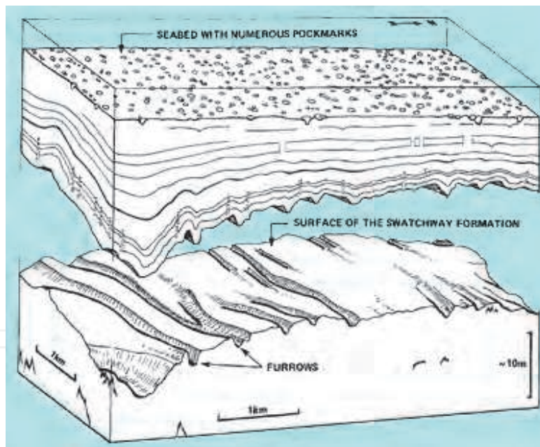
Fig. 12. Pockmarks in the Forties area, central North Sea (Based on Hovland and Judd, 1988).
