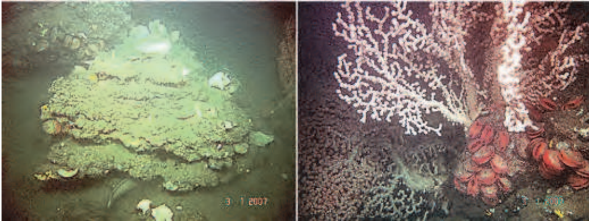
Fig. 10. Left: Large carbonate rock, a methane derived authigenic carbonate (MDAC). It serves as foundation for the Paragorgians and Acesta organisms seen in the right image. Notice the dense cluster of about 10 cm long Acesta excavata bivalves attached to the stems of the large gum corals and to the underlying MDAC-rock (From Hovland et al., 2010).
