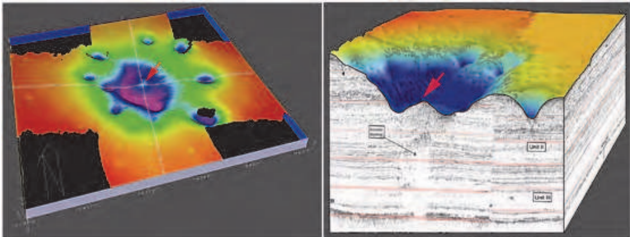
Fig. 9. The left image is a perspective view of a portion of the seafloor at the Troll field mapped at high resolution with ROV. It shows one central (old) 'parent pockmark' in the middle and eight of the other smaller 'satellite pockmarks' surrounding it. Right: Another view of the same features with enhanced vertical scale combined with high resolution SBP-data across the pockmarks. This drawing is made as a composite image based on real sub bottom profiler and bathymetric data from the actual location. The sides of this diagram are about 800 m, by 600 m, by 30 m. The red arrow points at the features seen in Fig. 10.
