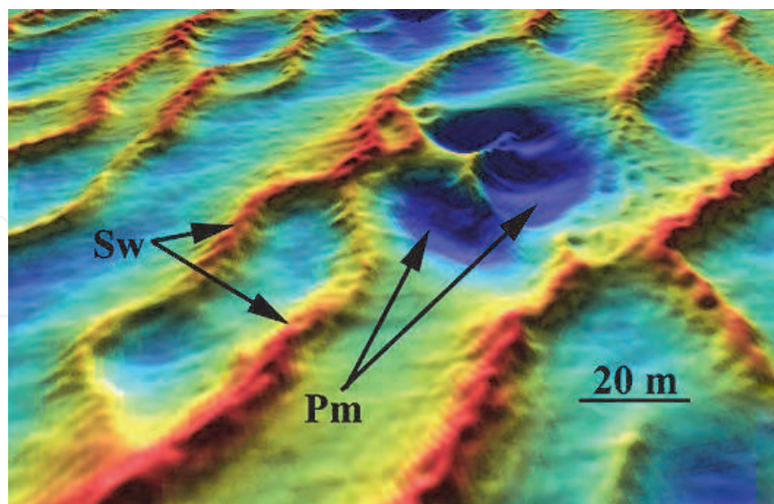
Fig. 21. A digital terrain model of a sandwave-field in the Southern North Sea. The regular sandwave pattern has clearly been disturbed by pockmark development (see text for further details). Sw=Sandwave, Pm=Pockmark. The highest sandwave crest is about 12 m above the 'normal' seafloor (greenish hue) and the deepest pockmark is about 2 m below that same depth (Based on Judd and Hovland, 2007).
