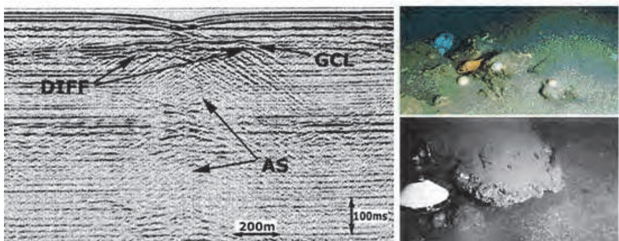
Fig. 6. The Scanner seep location is within a 22 m deep pockmark crater in the Witch Grounds of the North Sea, not far from the Forties field. The left image is a reflection seismic record showing reservoir gas (GCL) residing immediately below the pockmark depression. "Diff" = acoustic diffractions, "AS" = acoustic shadow zones. To the right are two images of the seafloor environment at the bottom of the pockmark. The lower one shows a white funnel (20 cm high), mounted on the ROV for gas sampling. Furthermore, there is a large MDAC rock adjacent to the bubbling gas stream being sampled (not visible). In the upper right photo, the red fish is about 20 cm long
