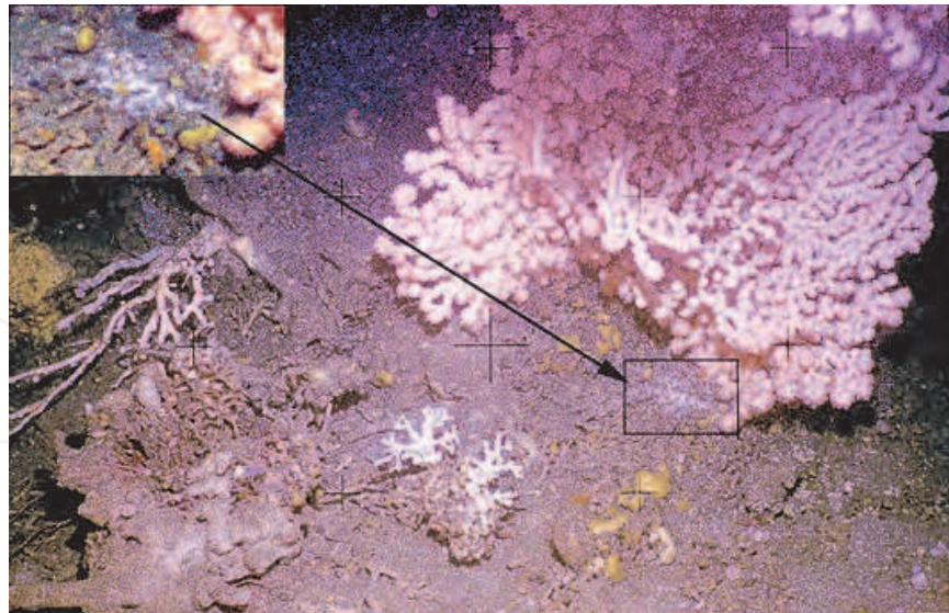
Fig. 16. A spectacular image of the seafloor, which was acquired in 1991 by use of ROV at the Onyx field (Block 6407/4, Hovland, 2008), near the seeps shown in the previous two figures. The arrowed insert image has been enlarged to show a white bacterial mat (see text for further explanation).
