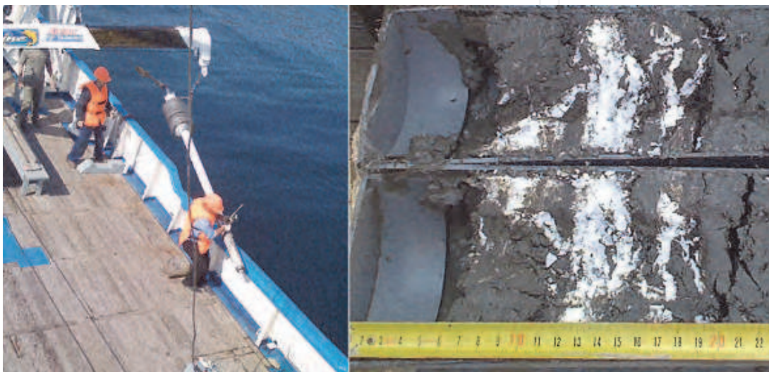
Fig. 24. The sampling of gas hydrates in Lake Baikal, 2010, was achieved by the use of a 800 kg heavy gravity corer, seen on the left being hoisted on board after having penetrated the seafloor, at 403 m water depth. After the clay-rich sediment core was split in two the result is seen on the right. There are veins and layers of pure gas hydrates inside the soft sediments.
