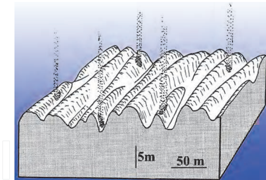
Fig. 15. A sketch showing how gas is suspected to flow out along linear ridges on the seafloor at the Onyx field off Mid-Norway. See text for further description and discussion (based on Hovland, 2008).
