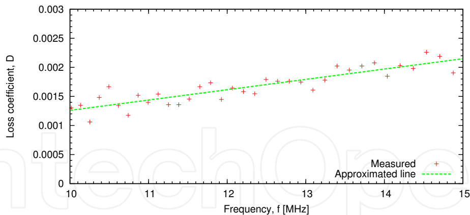
Fig. 8. Characteristics of the capacitor loss coefficient
