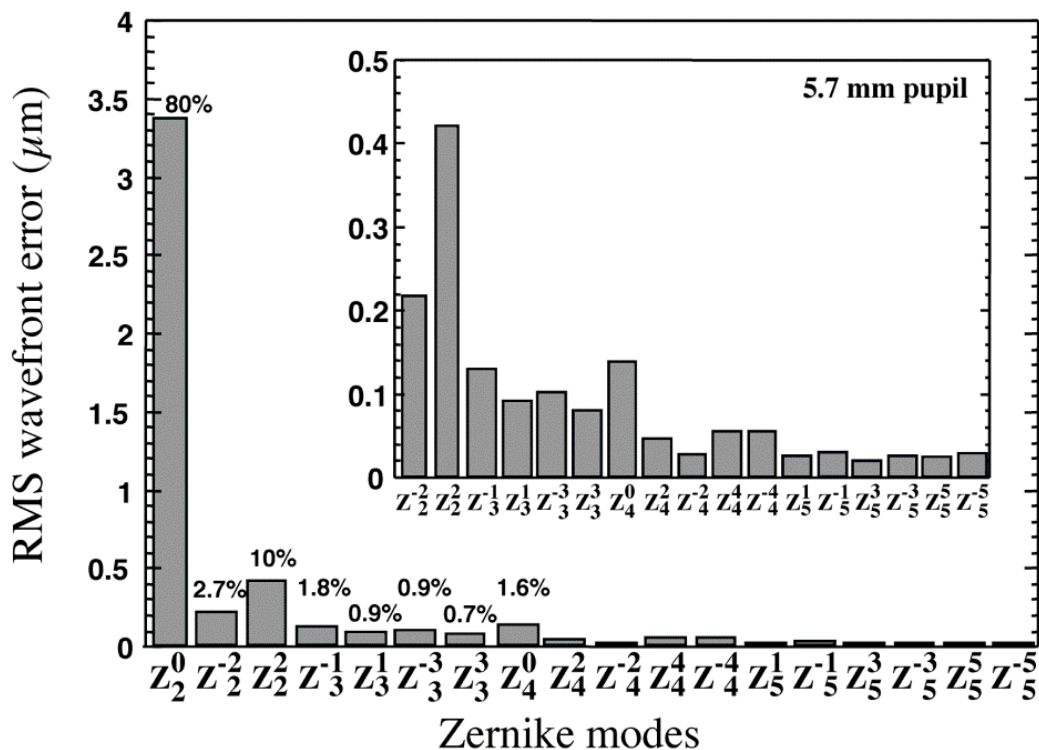
Fig. 4. The wavefront aberration decomposed into Zernike polynomials for a large human population (Porter et al, 2001) over a 5.7 mm pupil. The majority of the aberration power is found in the low order modes, i.e. defocus ( Z_2^0 ) and astigmatism ( Z_2^{-2} and Z_2^2 ). The percentages above the first eight modes indicate the percentage of the total wavefront variance. Note: the Zernike order follows that of Noll (1976). Reproduced with permission from the Optical Society of America (OSA).
