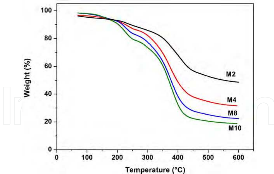
Fig. 4. TGA and DTG (insert) curves of hybrids prepared with MMA/MPTS ratios of 2 (M2), 4 (M4), 8 (M8) and 10 (M10).
