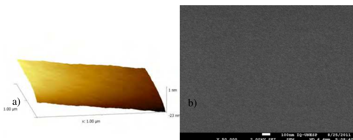
Fig. 10. Flat and featureless surface observed by a) AFM and b) FEG-SEM of the hybrid film prepared with a [\text{C}_{\text{CNT}}]/[\text{C}_{\text{CNT}} + \text{Si}] molar concentration of 5% (M4_5).
