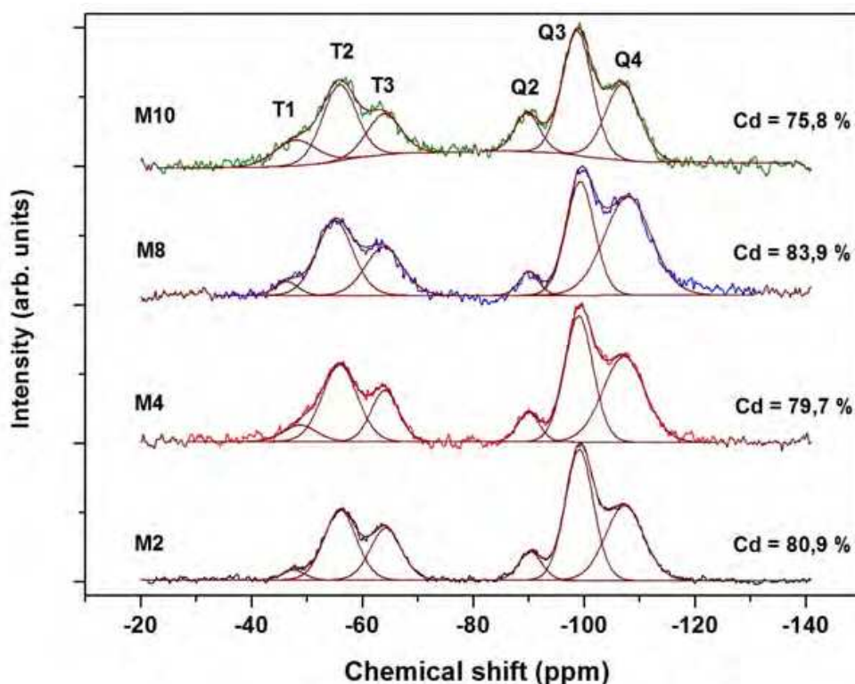
Fig. 3. 29 Si NMR spectra of hybrids prepared with MMA/MPTS ratios of 2 (M2), 4 (M4), 8 (M8) and 10 (M10).
