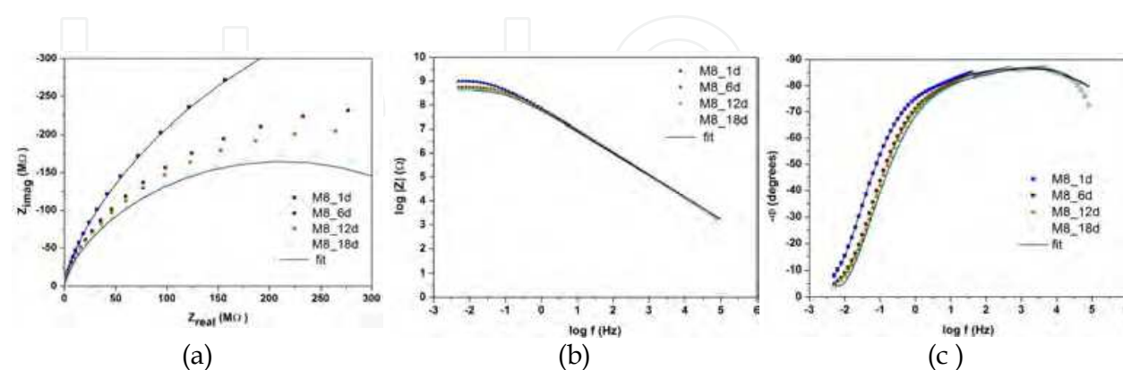
Fig. 7. Complex plane impedance (a), modulus impedance (b) and phase (c) plots of hybrids prepared with MMA/MPTS ratios of 8 (M8) after exposure of up to 18 day in unstirred and naturally aerated 3.5% NaCl solution. (The small discontinuities of \theta vs. \log f mark the change of the measurement range of the instrument.)
