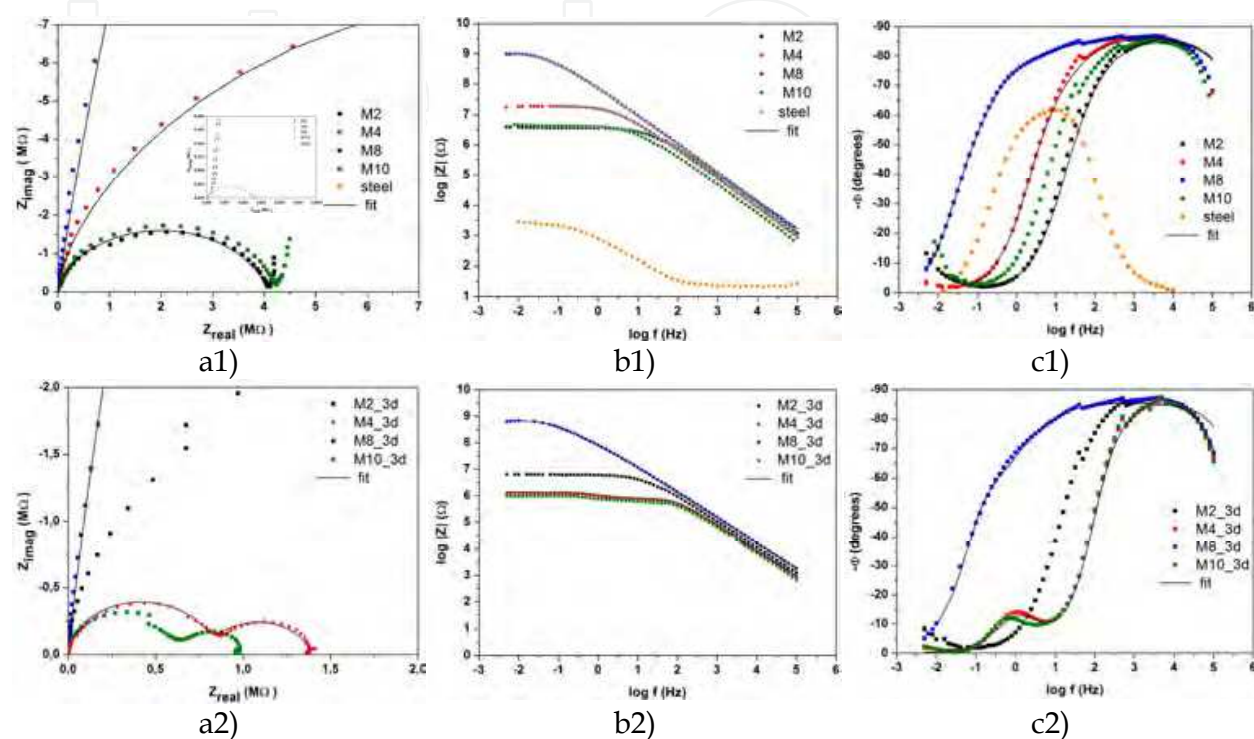
Fig. 6. Complex plane impedance (a), modulus impedance (b) and phase (c) plots of bare carbon steel and hybrids prepared with MMA/MPTS ratios of 2 (M2), 4 (M4), 8 (M8) and 10 (M10) after exposure of 1 day and 3 days in (1) unstirred and naturally aerated 3.5 % NaCl and (2) 0.05 mol L -1 NaCl + 0.05 mol L -1 H 2 SO 4 solutions, respectively. (The small discontinuities of \theta vs. \log f mark the change of the measurement range of the instrument.)
