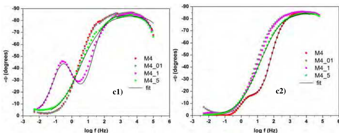
Fig. 15. Complex plane impedance (a), modulus impedance (b) and phase (c) plots of bare carbon steel and hybrids prepared with a MMA/MPPTS a ratio of 4 containing CNTs with [C_{CNT}]/[C_{CNT}+ Si] molar concentrations of 0% (M4), 0.1% (M4_01), 1.0% (M4_1) and 5% (M4_5) after exposure of 1 day in (1) unstirred and naturally aerated 3.5 % NaCl and (2) 0.05 mol L -1 NaCl + 0.05 mol L -1 H 2 SO 4 solutions. (The small discontinuities of \theta vs. log f mark the change of the measurement range of the instrument.)
