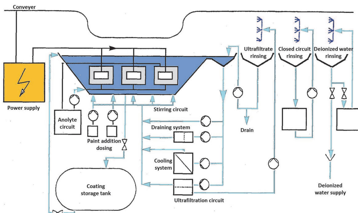
Fig. 2. Schematic representation of industrial process of cathoporesis.
