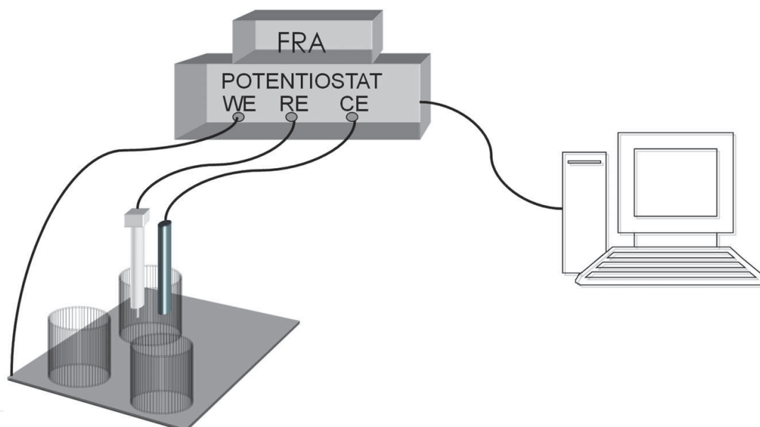
Fig. 3. Schematic representation of the electrochemical cell
