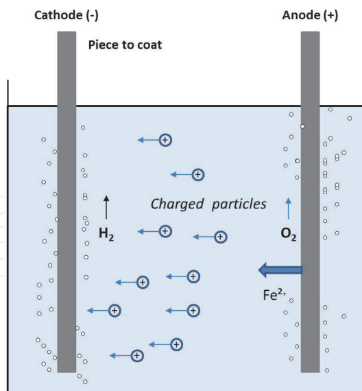
Fig. 1. Schematic representation of cathodic deposition.
