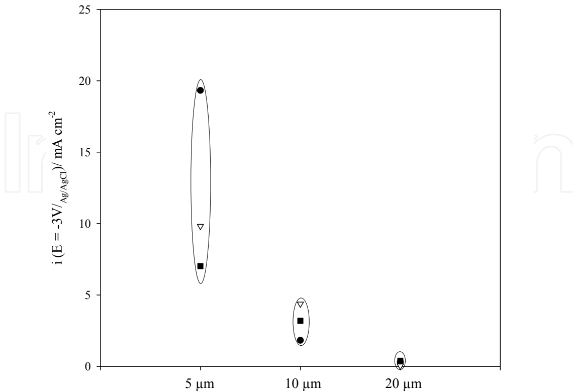
Fig. 17. Current density at a cathodic potential of -3V/Ag/AgCl for different coat-1% thicknesses (measured on the flat part) deposited on knife blades.
