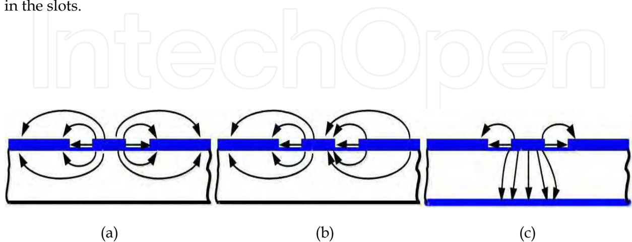
Fig. 2. Schematic electrical field distribution in coplanar waveguide: (a) desired even mode, (b) parasitic odd mode, and (c) parasitic parallel plate mode
