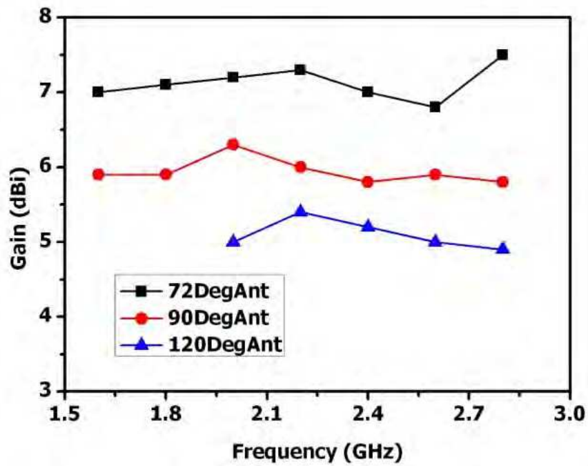
Fig. 32. Measured gains of the fabricated antennas
