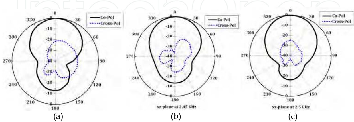
Fig. 35. Measured radiation patterns for the CPW-fed slot antenna with the metasurface in E -plane. (a) 2400 MHz, (b) 2450 MHz and (c) 2500 MHz
