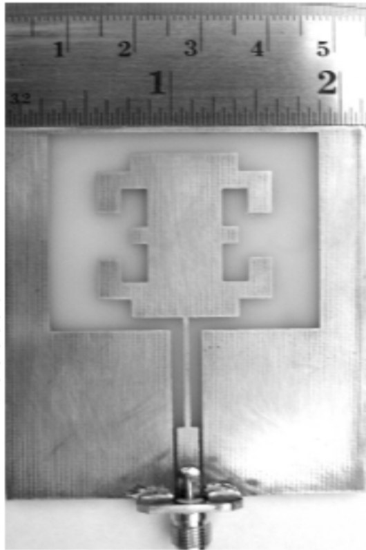
Fig. 23. (a) Configurations of the proposed fractal slot antenna and (b) photograph of the prototype
