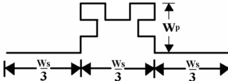
Fig. 24. The initial generator model for the proposed antenna
