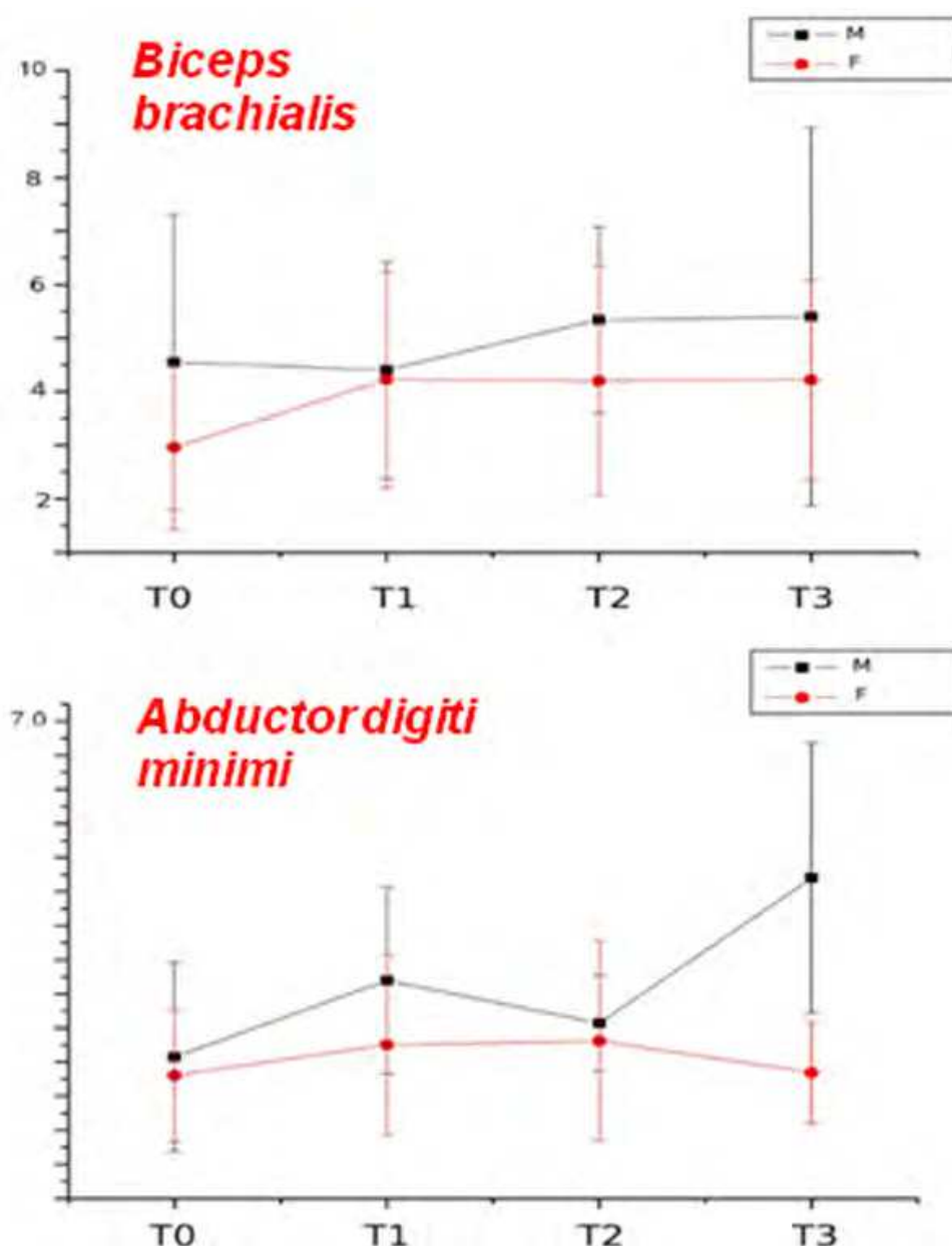
Fig. 5. MUP amplitude at T0 did not show any significant difference between females and males, both in spinal and bulbar form, even if a bit higher in males ( p > 0.05 ; Sartucci et al., personal data).
