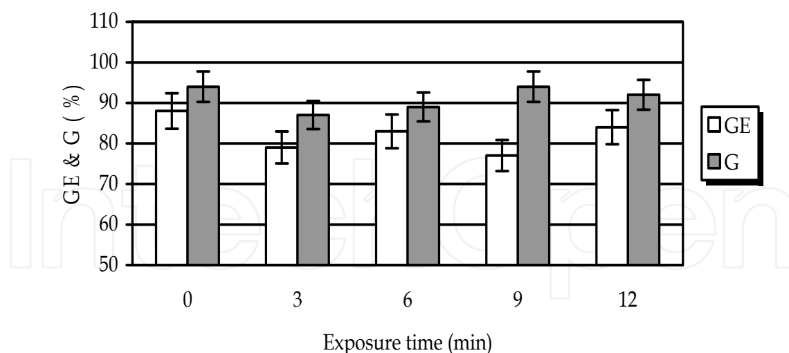
Fig. 1. Germination energy (GE) and germination (G) of lentils seeds exposed to static magnetic field.
