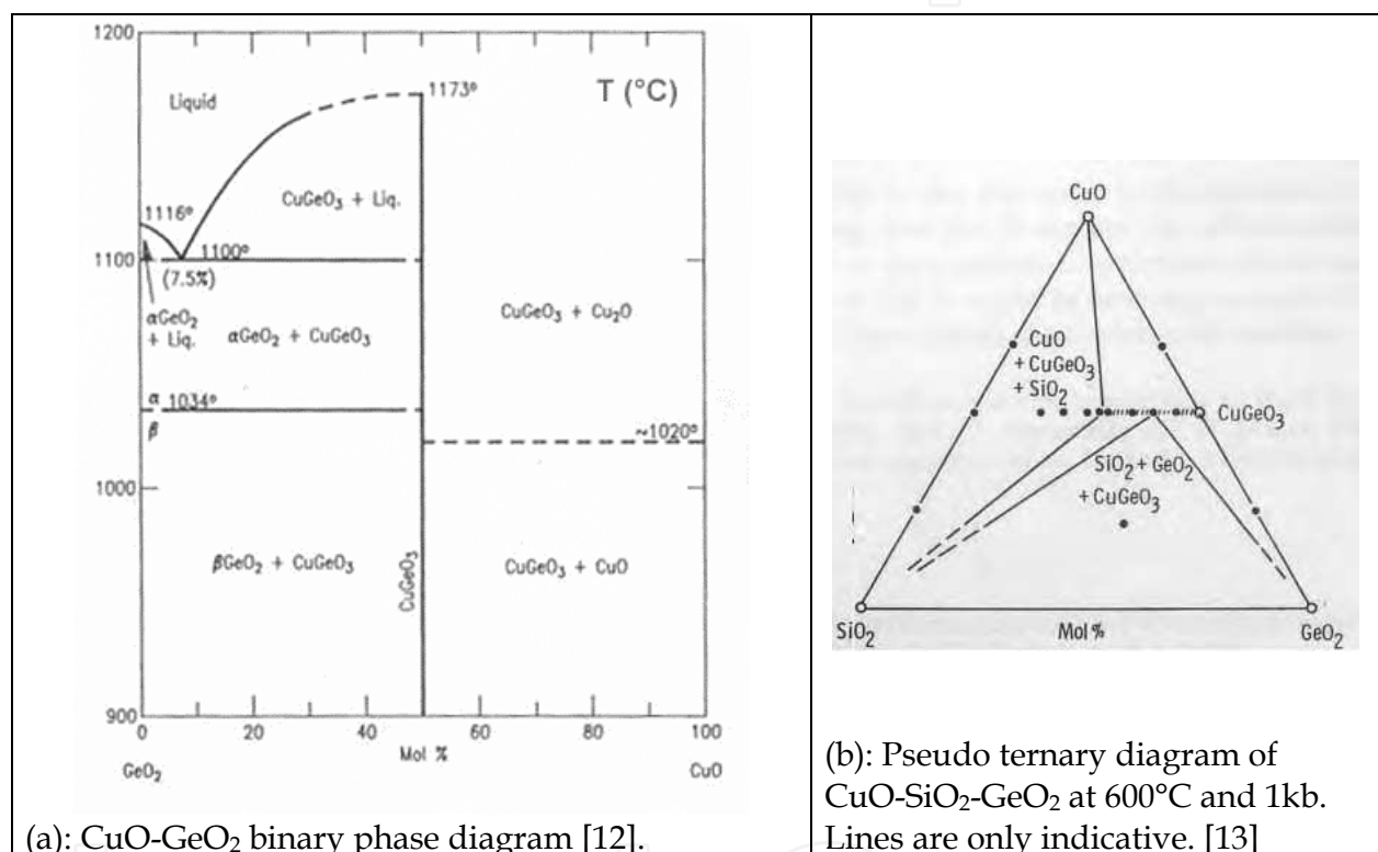
Fig. 3. Phase diagrams for CuGeO 3 .
