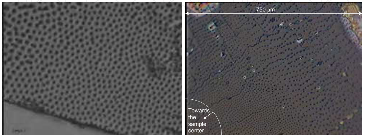
(a) Central region of \text{Cu}_{1.0}\text{Ge}_{0.9}\text{Si}_{0.1}\text{O}_{3.0} , 1mm/h (UPS417b) Precipitate distance is 4.1 microns, their size is 2.5 microns
