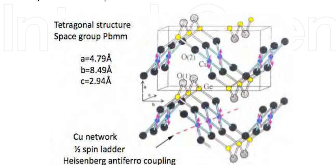
Fig. 2. \text{CuGeO}_3 crystallographic stacking.
