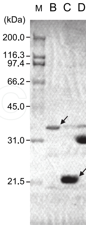
Fig. 1. SDS-PAGE analysis of RmlBCD. Eight \mu l of each cell-free supernatant from E. coli cells expressing rmlB (lane B), rmlC (lane C) or rmlD (lane D) was analyzed, and contained 0.8, 4.0 or 4.0 \mu g, respectively, of the deduced product (indicated by arrows). M, molecular weight markers.
