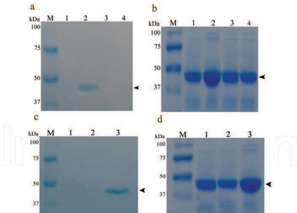
Fig. 1. SDS-PAGE gel (12% polyacrylamide) analysis of isolated surface proteins of Lactobacillus acidophilus ATCC 4356 at: a) mid-log phase ( OD_{600}= 0.4 ) and b) exponential growth phase ( OD_{600}= 0.7 ) under pH stress (lane 1, control; lane 2, pH 5; lane 3, pH 6; lane 4, pH 7). c) mid-log phase ( OD_{600}= 0.4 ) and d) exponential growth phase ( OD_{600}= 0.7 ) under heat stress (lane 1, control; lane 2, 30 °C; lane 3, 45 °C). M, Protein marker.
