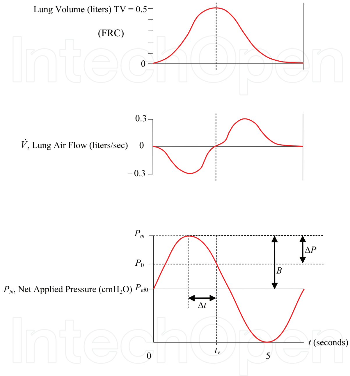
Fig. 4. Lung ventilatory model data shows air-flow ( \dot{V} ) and volume ( V ) and net pressure ( P_N ). Pause pressure ( P_0 ) occurs at t_v , at which the volume is maximum (TV = tidal volume). \Delta t is the phase difference between the time of maximum volume and peak pressure ( P_m ). It is also the time lag between the peak and pause pressures. B is the amplitude of the net pressure waveform P_N applied by the ventilator. This P_N oscillates about P_{el0} with amplitude of B . The difference between peak pressure P_m and pause pressure P_0 is \Delta p . This figure is adopted from our work in Ref [3].
