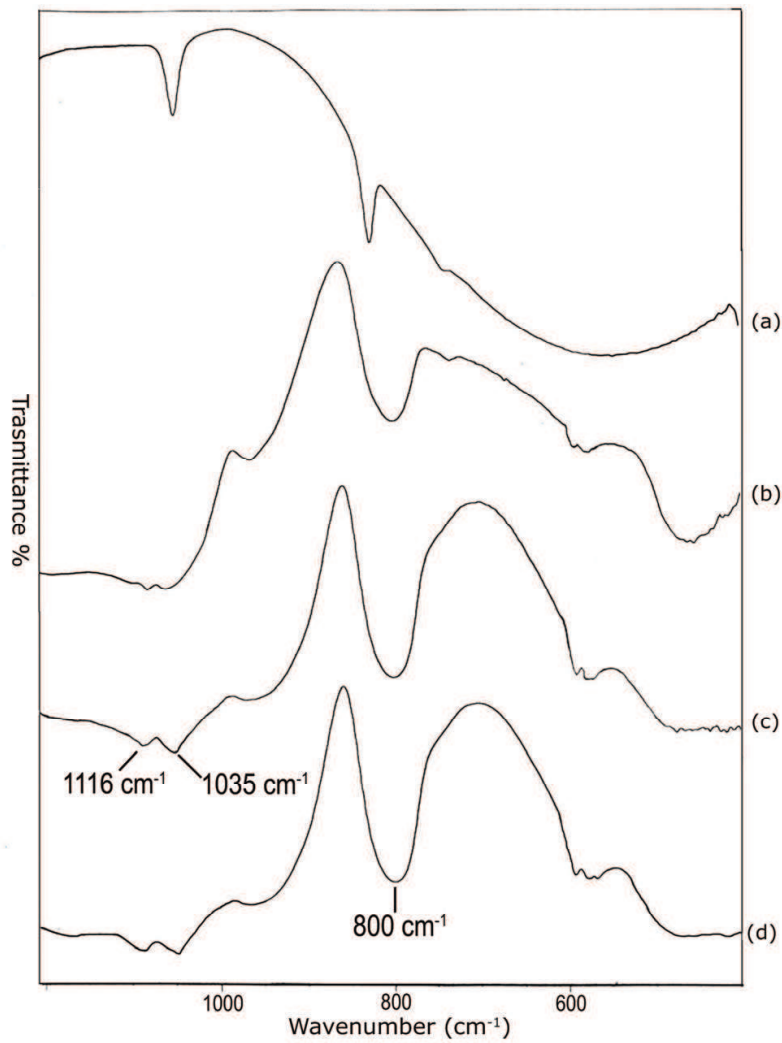
Fig. 15. FTIR spectra of \text{SiO}_2/\text{PCL} gel samples after different times of exposure to SBF: (a) not exposed; (b) 7 days exposed; (c) 14 days exposed; (d) 21 days exposed.
