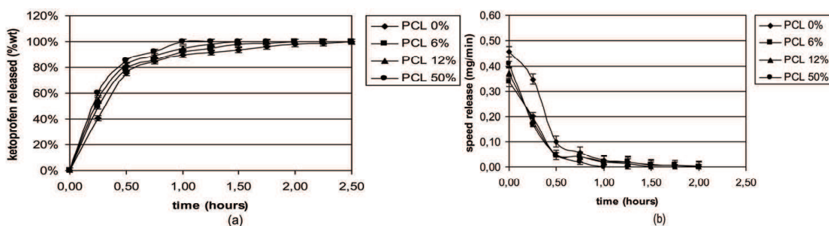
Fig. 20. (a) Time-dependent drug release plot for \text{SiO}_2 + PCL (0, 6, 12, 50% wt) + ketoprofen 15% at 37^\circ\text{C} in SBF solution; (b) Time-dependent drug release rate plot for \text{SiO}_2 + PCL (0, 6, 12, 50% wt) + ketoprofen 15% at 37^\circ\text{C} in SBF solution.
