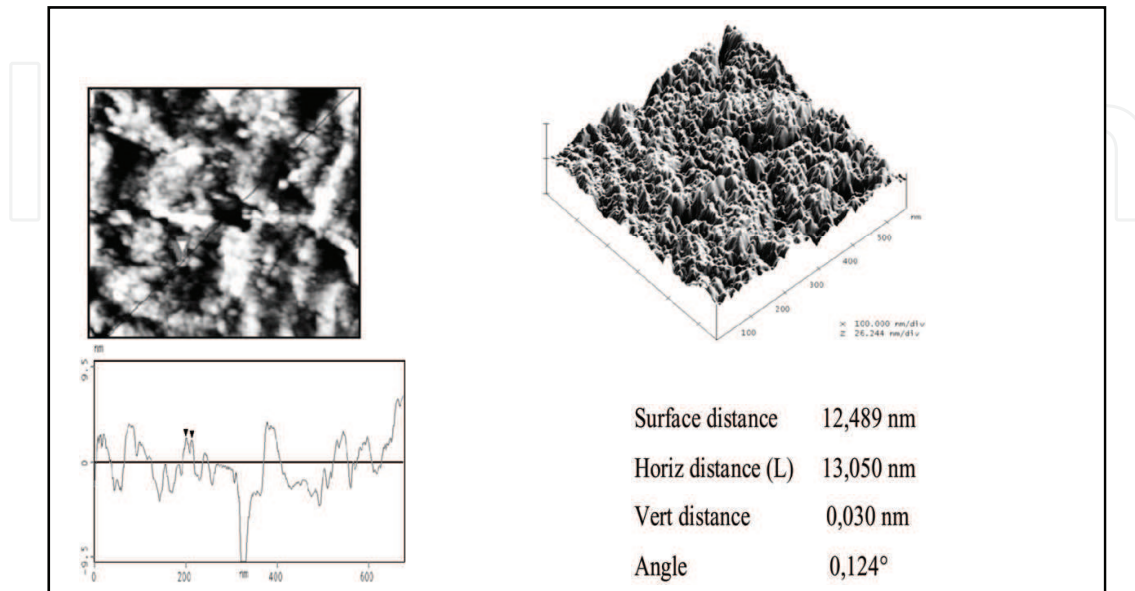
Fig. 14. AFM image showing the microstructure of SiO 2 /PCL gel.
