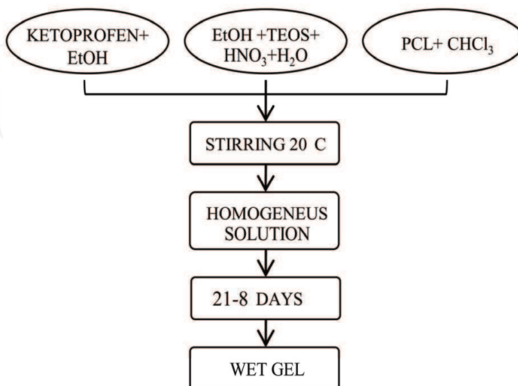
Fig. 7. Flow chart of SiO_2/PCL gel synthesis.
