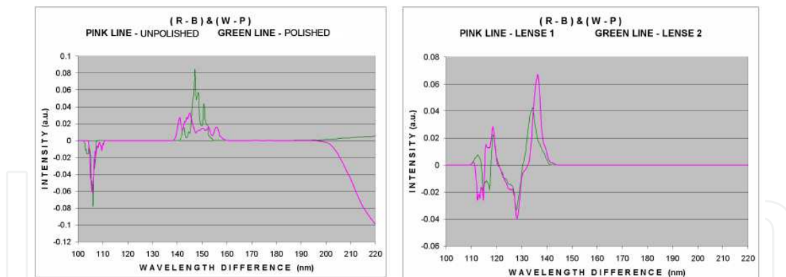
Fig. 10. Opto-Magnetic Fingerprint diagrams. Image on the left: overlapped OMF diagrams of two differently processed CLs that show different behaviour in the wavelength difference range of 130–150nm and sensitivity to changes in surface qualities. Image on the right: overlapped OMF diagrams of two identically processed CLs that show minor change in diagrams and surface qualities.
