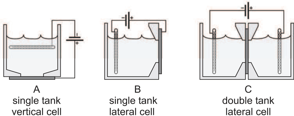
Fig. 4. Illustration of various types of anodization cells used to fabricate porous silicon wafers. Figure reproduced with permission from Gaburro, 2005.
