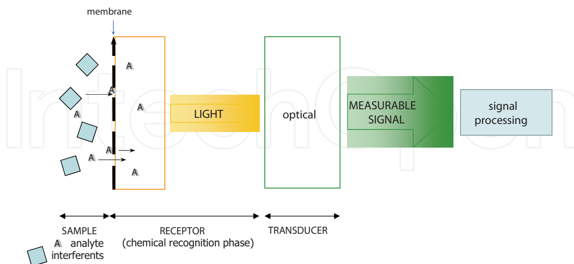
Fig. 1. Schematic representation of the composition and function of an optical chemical sensor
