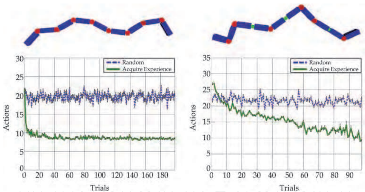
Fig. 4. Structure RRRRRRRR (eight degrees of freedom) plus learning curve and baseline on the left panel as well as structure RRPRRRPR (nine degrees of freedom) on the right panel.
