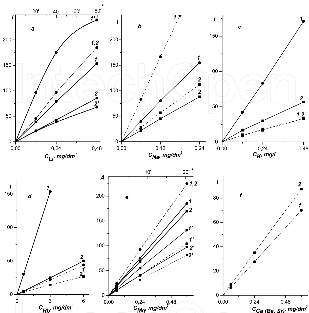
Fig. 5. Effect of H_3PO_4 on emission analytical signals ( I ) of alkali and alkali-earth elements (a, b, c, d, f) and absorption signals (A) of Mg (e) in acetylene-air (---), acetylene - nitrous oxide (- · - · -), propane-butane - nitrous oxide (- - -). Curves 1, (1') - model solution of element; 2, 2' - element + H_3PO_4 . *The burner is perpendicular to the optical axis
