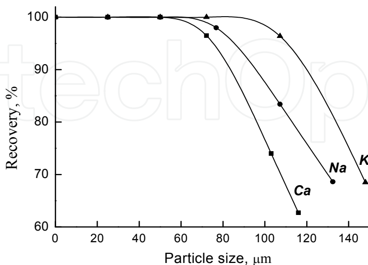
Fig. 7. Effect of \alpha -Al 2 O 3 particle size on the recovery of Na, K and Ca
