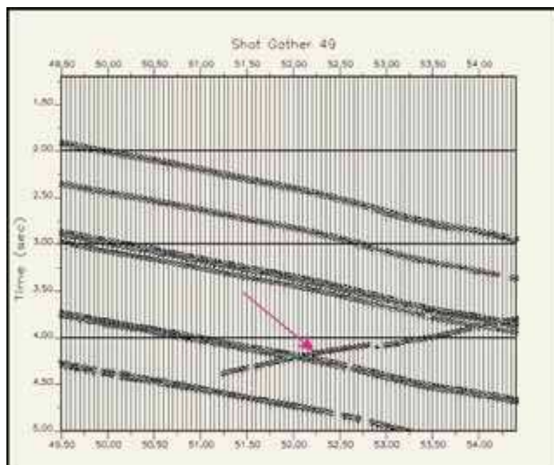
Fig. 10. Synthetic shot gather record at x=49.5\text{km} of Zagros model shown in fig. 7. Maximum offset is 4500m. The event indicated by the arrow represent a nonhyperbolic event in the shot gather record (Alaei, 2005)
