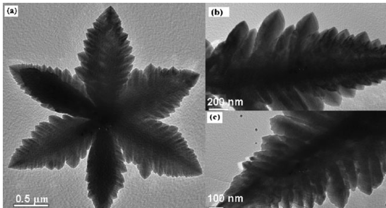
Fig. 13. TEM image of dendritic \alpha - \text{Fe}_2\text{O}_3 .
