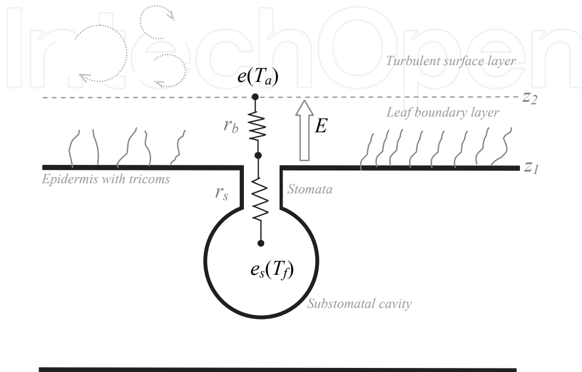
Fig. 2. Schematic picture of the transpirative process from a leaf. The symbols are explained in the text.
