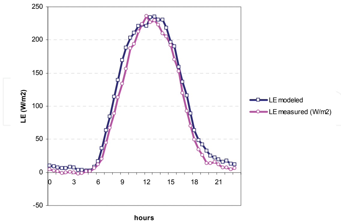
Fig. 6. Mean daily course of the modeled \lambda E compared to the measured one. All the available hourly measurements were considered ( n=3914 )
