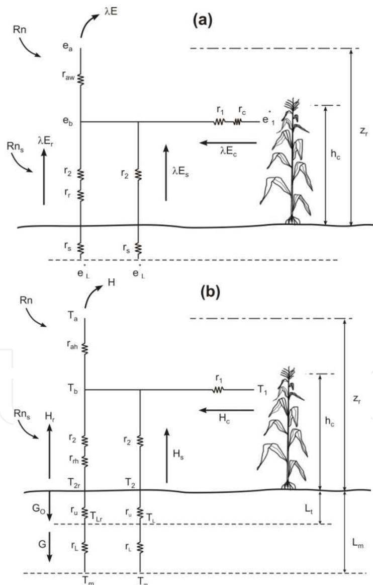
Fig. 2. Schematic resistance network of the Surface Energy Balance (SEB) model a) Latent heat flux and b) Sensible heat flux.
