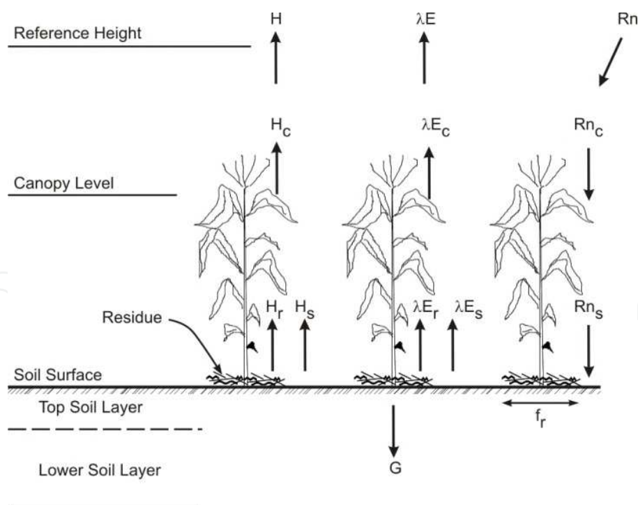
Fig. 1. Fluxes of the surface energy balance model (SEB).
