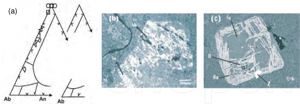
Fig. 15. Welded tuff: (a) diagram Ab-Or-An (electron microprobe and scanning electron microscope) = matrix, ♦ = rim, Δ = inter, ▽ = core, + = bright, x = dark, O = in Mt. (b) Photomicrography of the heterogeneous alkali feldspar crystalloclast corroded by the matrix (analyzed through the electron microprobe); (c) Photomicrography of the Ti-rich magnetite crystalloclast altered to ilmenite (Il), rutile (Ru) disposed according to twinning and/or cleavages with zircon inclusions (Z) and replaced by sanidine (Sa) (scanning electron microscope).
