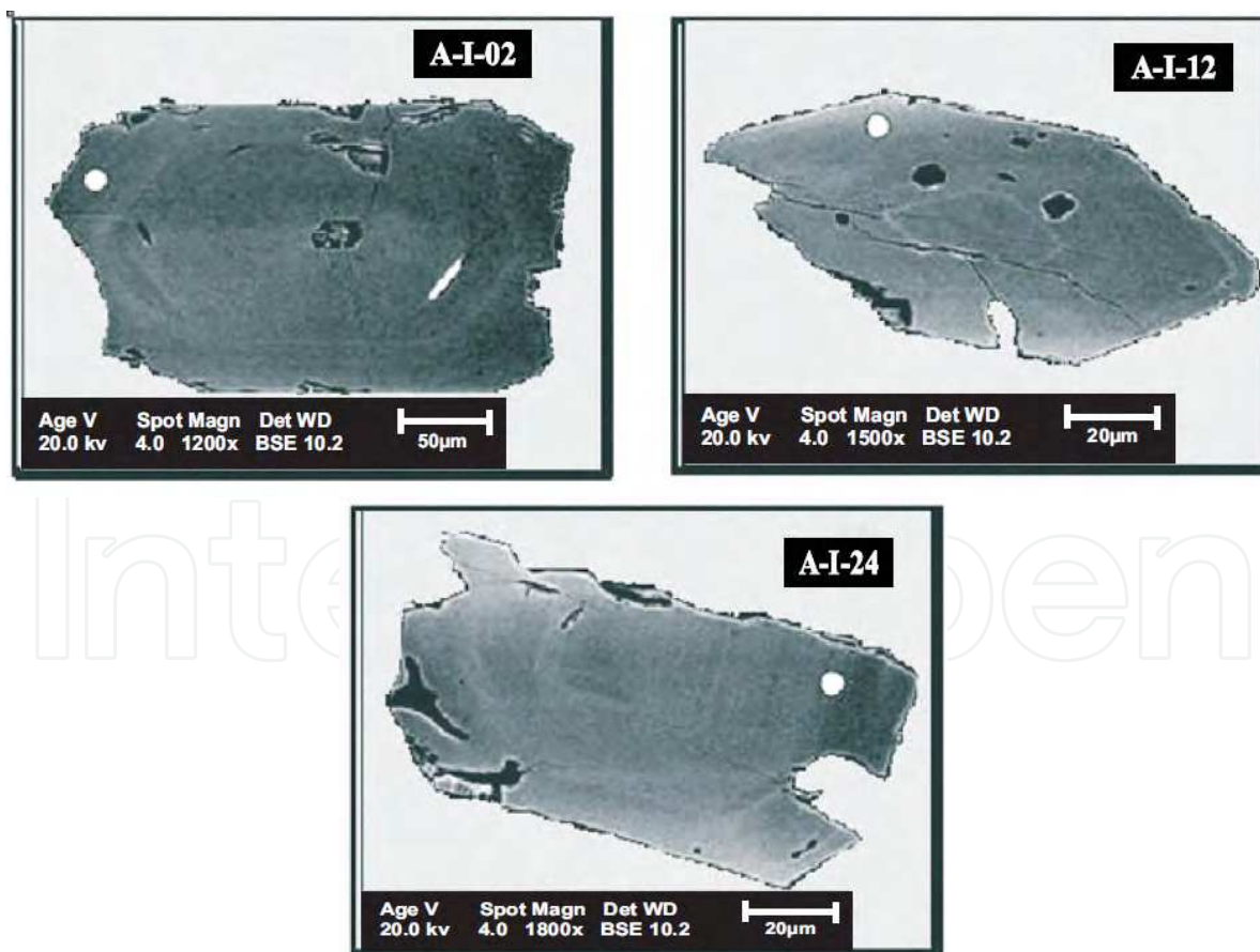
Fig. 9. Zircons microphotographies that defined the 553 \pm 5.4 Ma age for Acampamento Velho Formation base. A-I-02 sample number, \bigcirc = spot showing the place where the analysis were realized in each zircon. Data showed in table 4.
