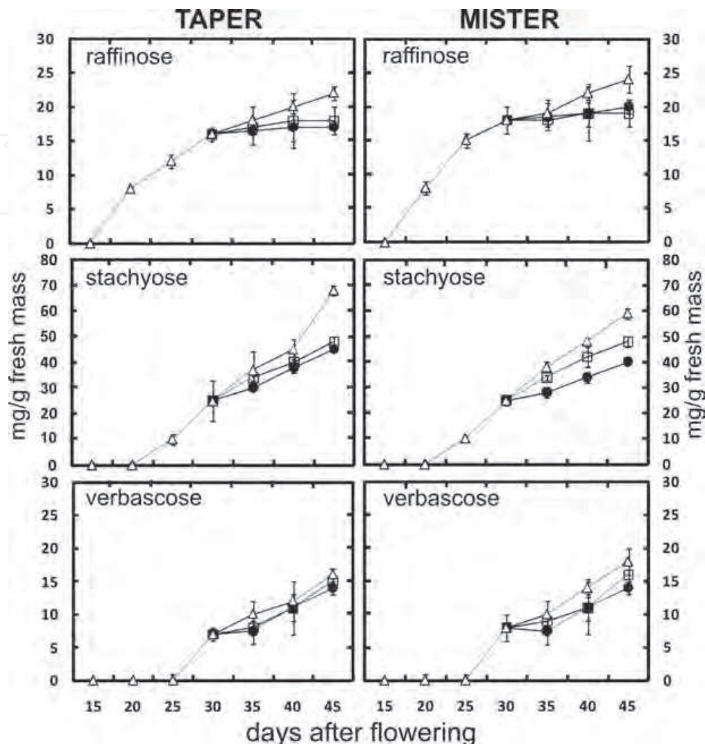
Fig. 6. Raffinose family oligosaccharides content in lupin seeds during maturation and after application of herbicides: Basta 200 SL and Roundup Ultra 360 SL. Data points represented the mean \pm SD for fifteen replicate samples - control ( \Delta ), Basta treatments ( \square ), Roundup treatments ( \bullet ).
