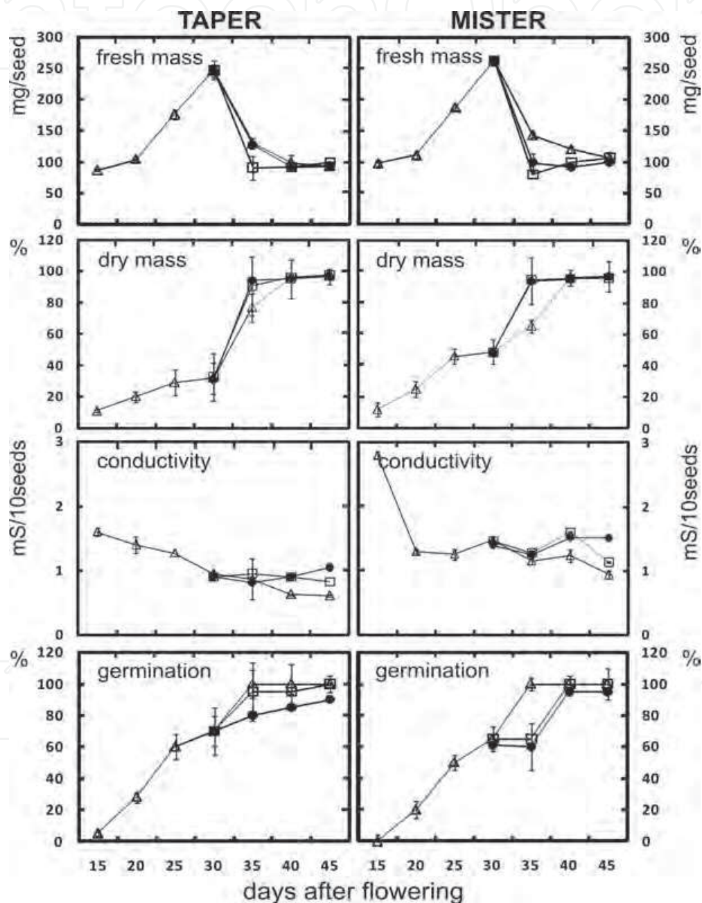
Fig. 3. Seed dry and fresh mass, conductivity and germination during maturation and after application of herbicides: Basta 200 SL and Roundup Ultra 360 SL. Data points represented the mean \pm SD for fifteen replicate samples - control ( \Delta ), Basta treatments ( \square ), Roundup treatments ( \bullet ).
