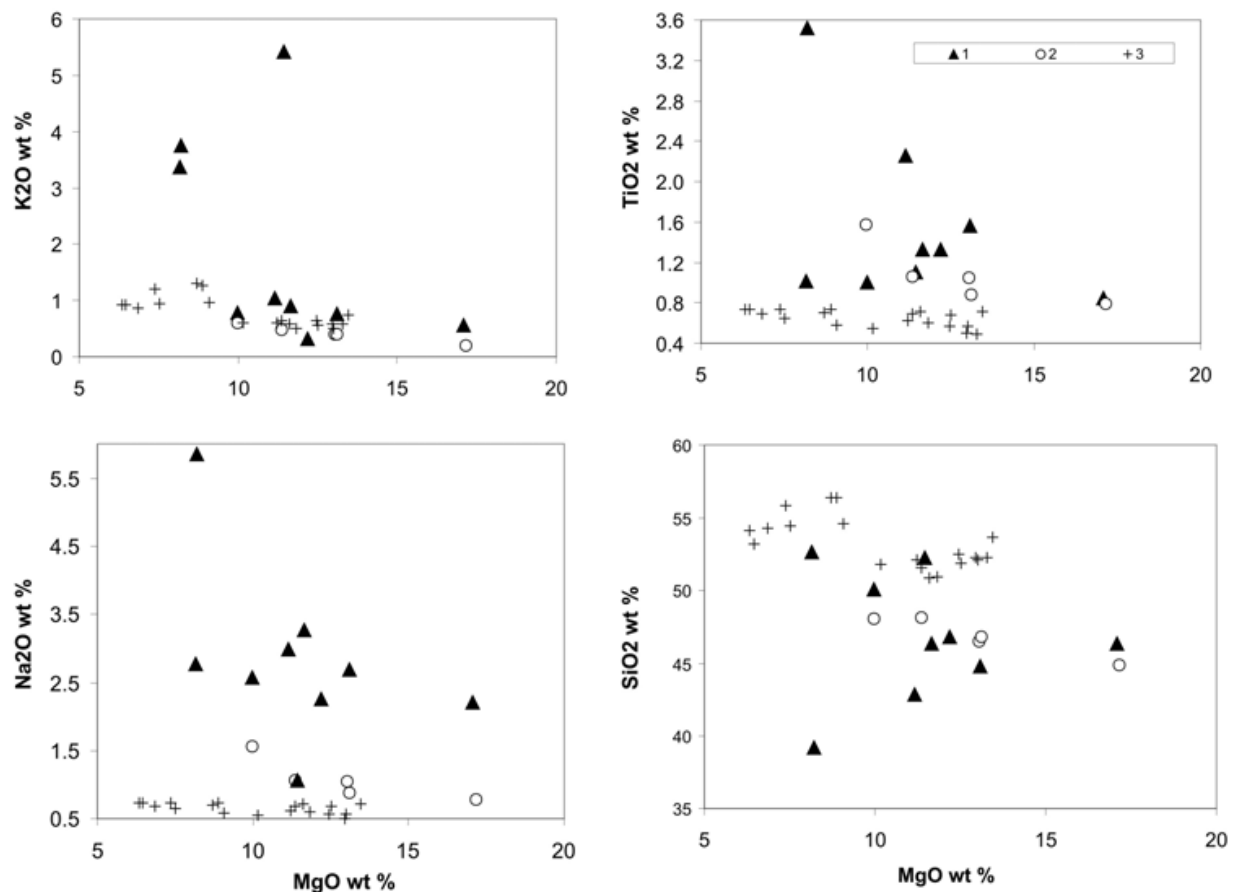
Fig. 2. Variations in major element contents for the Schirmacher dolerites. (1) Dolerites of the Schirmacher Oasis (Table 1), (2) dikes of the Muren region of DML after (Vuori & Luttinen, 2003), and (3) ancient anorthosite dikes from the Schirmacher Oasis region (Belyatsky et al., 2002).
