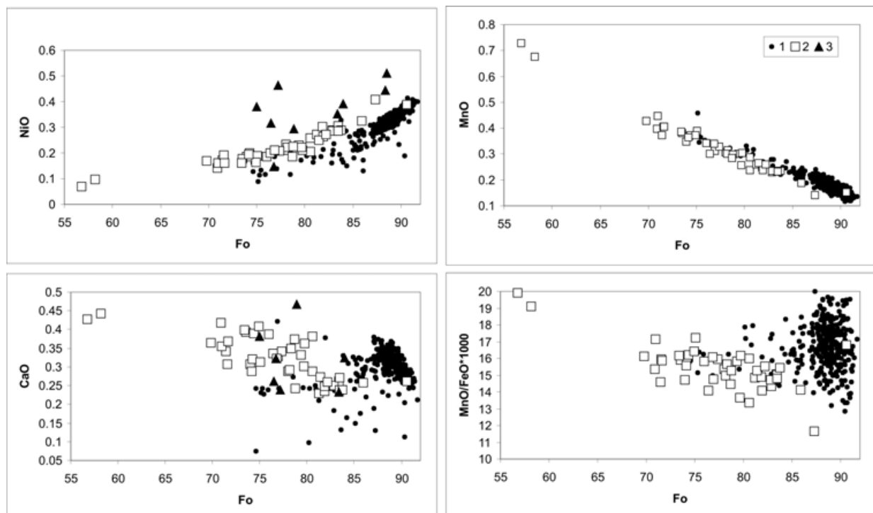
Fig. 3. Contents of NiO, CaO, and MnO in olivines from the Schirmacher Oasis dikes as a function of forsterite mole percentage. Olivines from (1) sample 47139-7, (2) sample 47225-7, and (3) DML basalts (Sushchevskaya et al., 2004).
