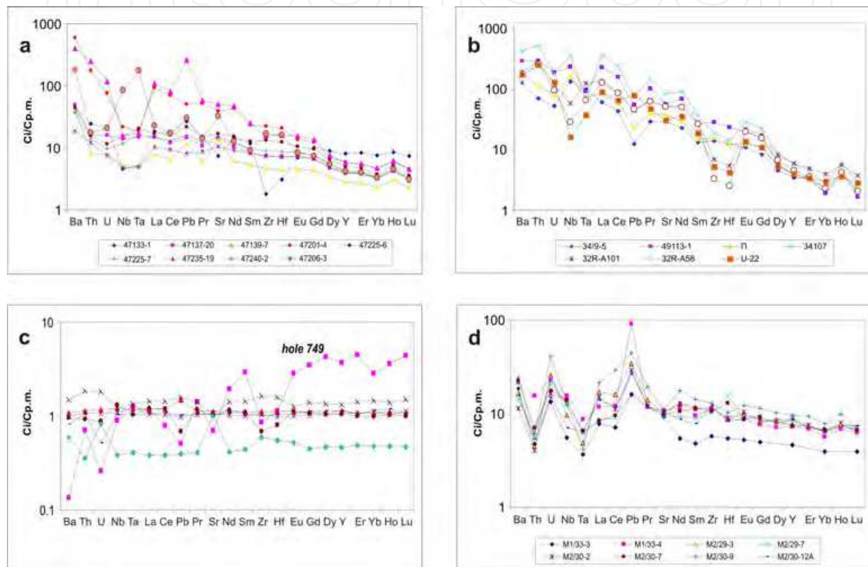
Fig. 7. Primitive mantle-normalized (Sun & McDonough, 1989) distribution of lithophile element patterns in the Schirmacher Oasis dolerites (a), Jetty Oasis alkaline picrites (b), Kerguelen Plateau tholeiites (Frey et al., 2000) (c) and the Afanasy Nikitin Rise tholeiites (Borisova et al., 2001) (d).
