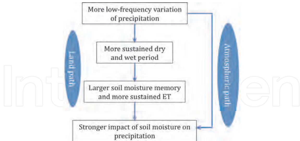
Fig. 5. Schematic of the impact of precipitation variability on soil moisture-precipitation coupling.
