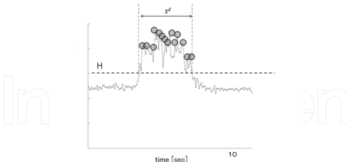
Fig. 5. A series of maximal values of the ARS during the muscular contraction periods in the BFT were extracted by our mathematical algorithm of the sensor output signal evaluation system.
