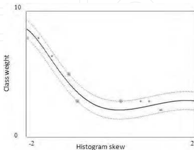
Fig. 3. Skew to class weight mapping
