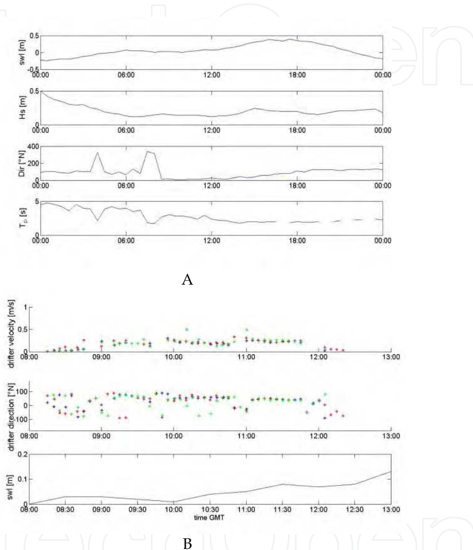
Fig. 6. A) Measured swl (top panel), significant wave height ( H_s ), direction and period ( T_P ). B), drifters' velocity (top panel), direction (central panel) and contemporary swl (bottom panel).
