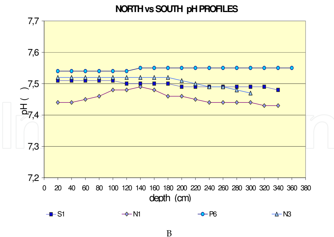
Fig. 12. A) Thermoaline and B) pH profiles at the beginning of the experiment at sections S1, N1, N3, P6 (see Fig.2).
