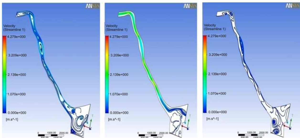
Fig. 5. Lines of transient currents in the Rio Matapi: a) low tide at t = 1h , b) end of the ebb at t = 5.5 h , c) reversal of the tide at t = 6h .
