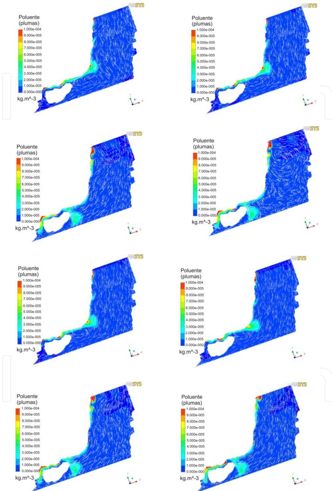
Fig. 4. Velocity and dispersion of pollutants in natural runoff - in the coast of the cities of Macapá and Santana. Representation of a semi-diurnal tidal cycle.
