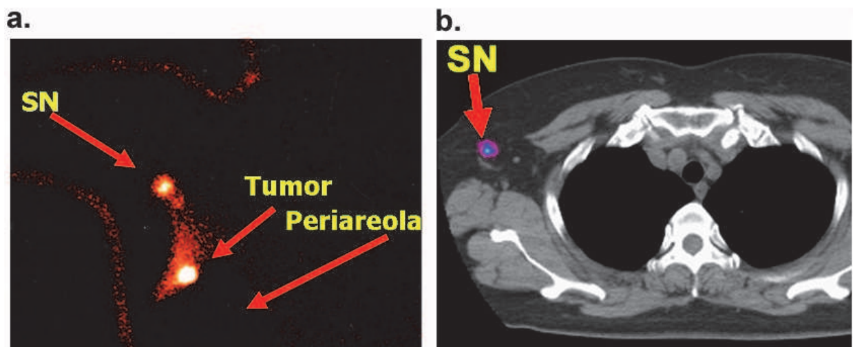
Fig. 5. Lymphoscintigraphy and SPECT-CT
