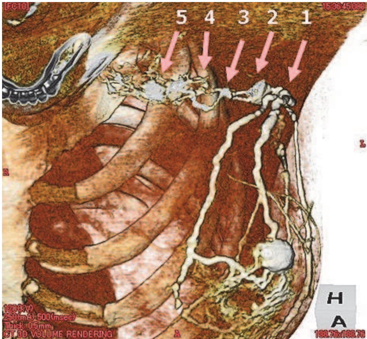
Fig. 3. Chronological examination of 3D-CT LG (Yamashita, 2009).
