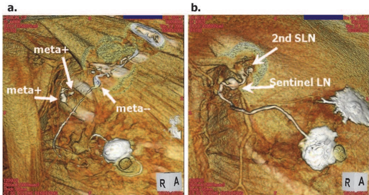
Fig. 4. Detection of SN metastasis (Yamashita, 2009).
