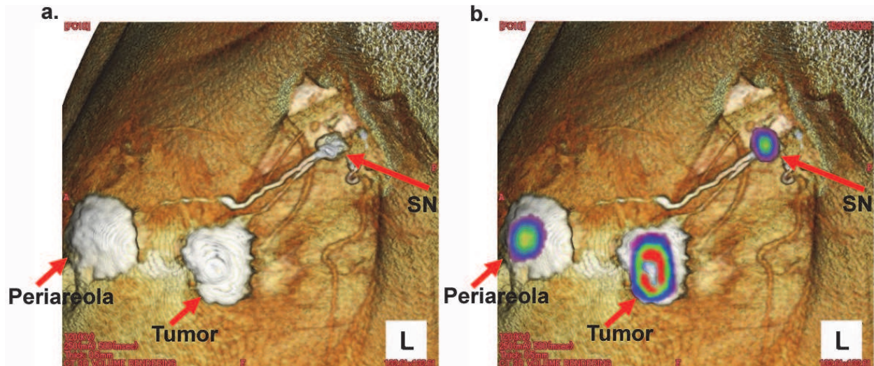
Fig. 6. 3D-CT lymphography and SPECT-fused 3D-CT LG
