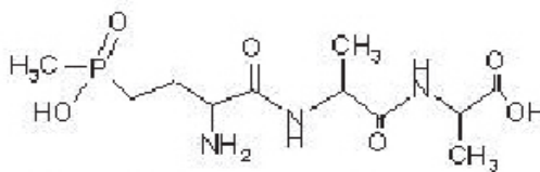
phosphinotricin-alanyl-alanine
