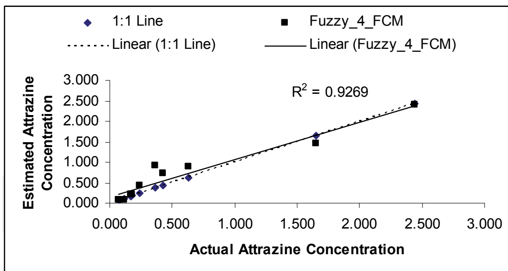
Fig. 7. Scatter plot of observed and Fuzzy_4_FCM Model predicted average monthly atrazine concentration for the testing period year 2001.
