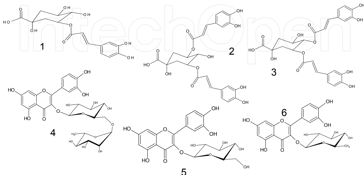
Fig. 5. Chemical structures of compounds from n -butanol fraction of leaf extract from A. trifoliatum : 1 = chlorogenic acid, 2 = 3,5-di- O -caffeoylquinic acid, 3 = 4,5-di- O -caffeoylquinic acid, 4 = rutin, 5 = isoquercetin, 6 = quercitrin.
