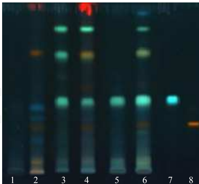
Fig. 3. TLC chromatogram of extracts from A. trifoliatum . Track : 1= root 95% maceration, 2= leaf 95% maceration, 3= root 75% refluxing, 4= leaf 75% refluxing, 5= root decoction, 6= leaf decoction, 7= standard chlorogenic acid, 8= standard quercetin, Stationary phase: silica gel GF254 Solvent system: ethyl acetate: acetic acid : formic acid : water 137: 11: 11: 26 Detection: NP-PEG spraying reagent / UV 366 nm.
