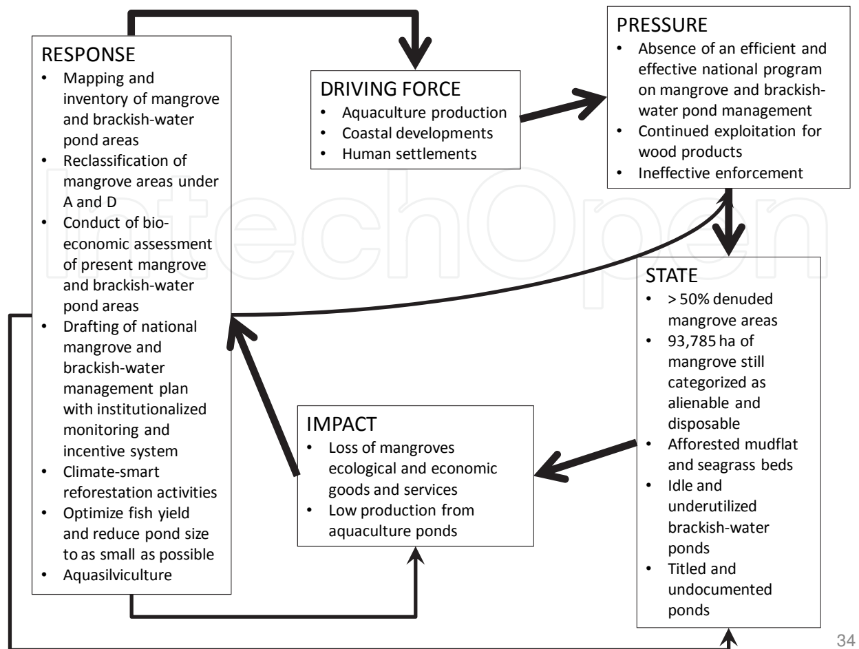
Fig. 4. DPSIR model on the state of mangrove forests and brackish-water ponds in the Philippines.
