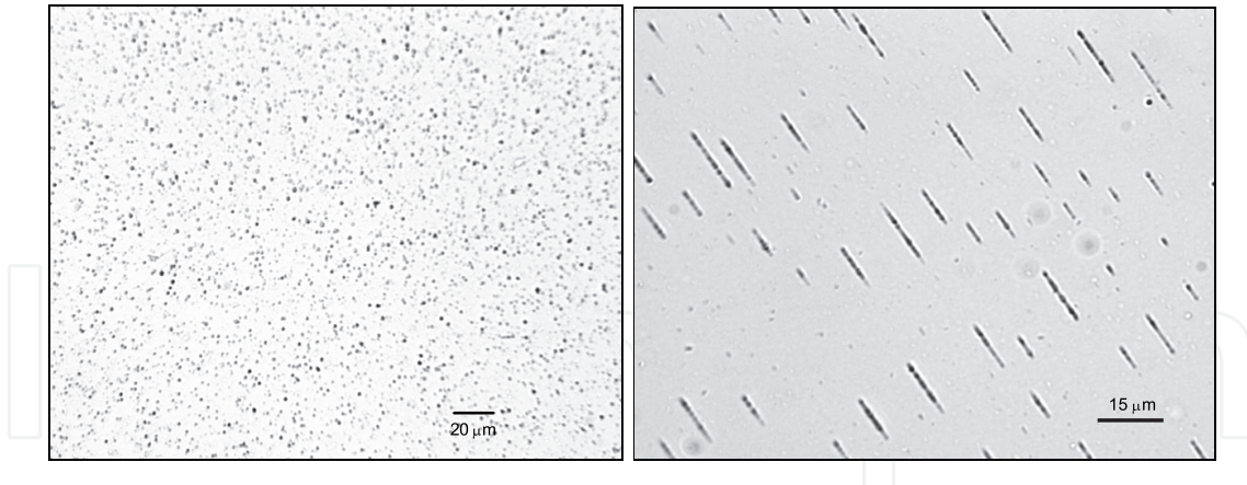
Fig. 3. Superparamagnetic microparticles observed when no external magnetic field is applied (Left) and when it is applied (Right).
