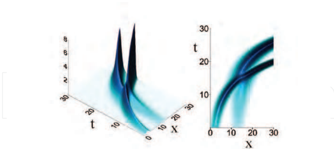
Fig. 8. Nonautonomous KdV solitons calculated within the framework of the model (71) after choosing the soliton management parameters \alpha = 0.15, \eta_{10} = 0.40, \eta_{20} = 0.75 . On the left hand side the temporal behavior is presented, while the corresponding contour map is presented on the right hand side.
