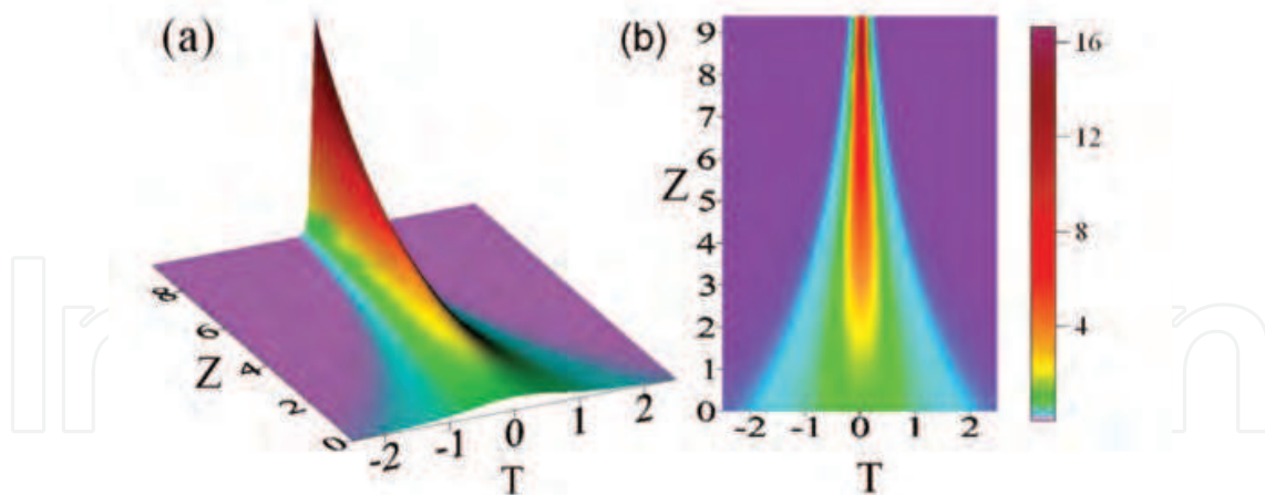
Fig. 2. Self-compression of nonautonomous soliton calculated within the framework of the model Eq. (46) after choosing the soliton management parameters c_0 = 0.05; \alpha = 0 and \eta_0 = 0.5 . (a) the temporal behavior; (b) the corresponding contour map.
