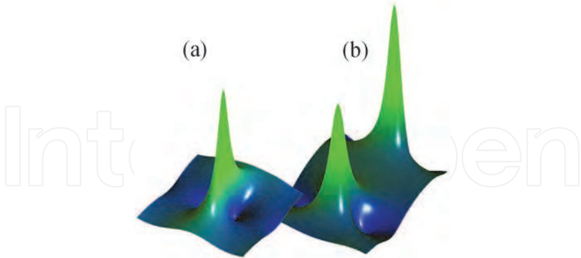
Fig. 6. Illustrative examples of the Peregrine soliton dynamics: (a) - classical Peregrine soliton calculated in the framework of the canonical NLSE model; (b) its behavior under linear amplification associated with continuous wind.
