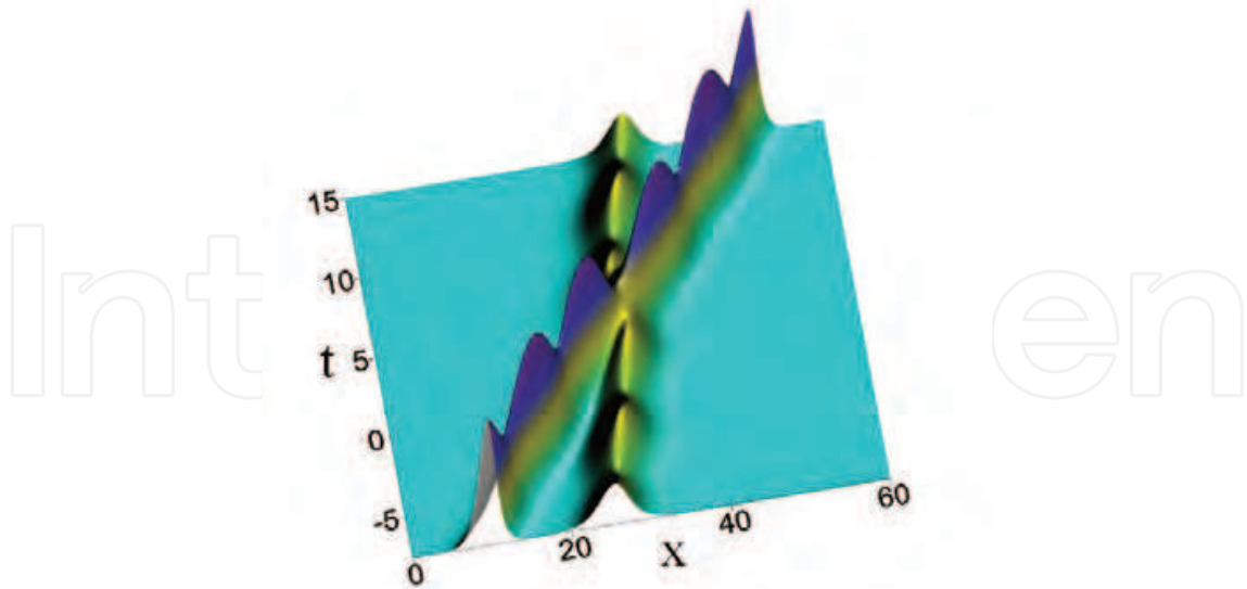
Fig. 9. Nonautonomous KdV solitons calculated within the framework of the model (72) after choosing the soliton management parameters \alpha = 2.0 , \beta = -0.25 , \eta_{10} = 0.40 , \eta_{20} = 0.75 .
