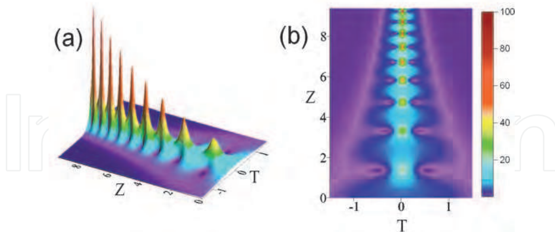
Fig. 3. Nonautonomous "agitated" breather (58) calculated within the framework of the model (46) after choosing the soliton management parameters c_0 = 0.25 , \eta_{10} = 0.5 , \eta_{20} = 1.5 . (a) the temporal behavior; (b) the corresponding contour map.
