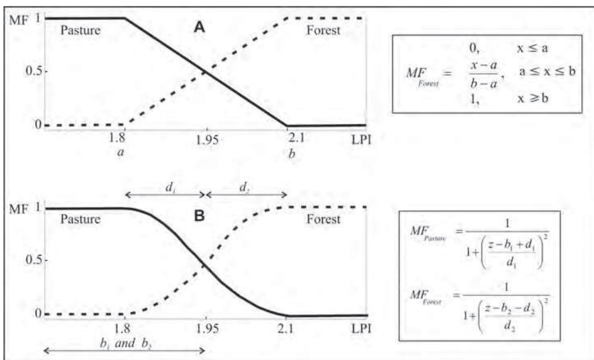
Fig. 4. Membership functions: (A) linear; (B) bell-shaped
