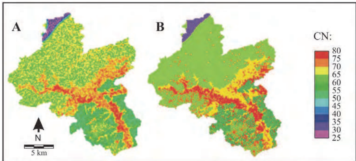
Fig. 8. CN maps obtained by the Fuzzy SCSCN model (A) and by the standard SCSCN model (B)
