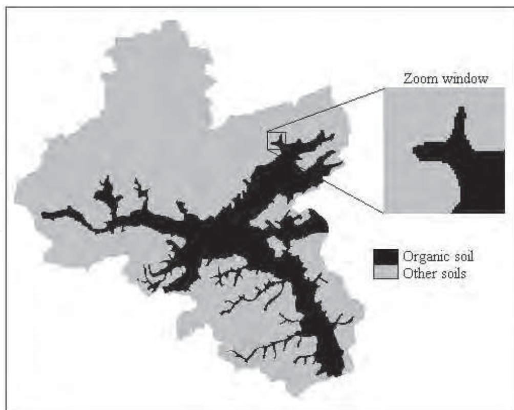
Fig. 7. Organic soil map with Boolean boundaries
