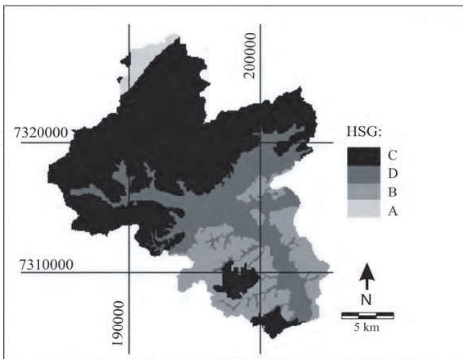
Fig. 3. Hydrologic Soil Group (HSG) map
