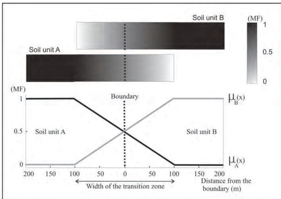
Fig. 5. Linear membership function and illustration of the methodology employed in the conversion of crispy soil data to fuzzy soil data
