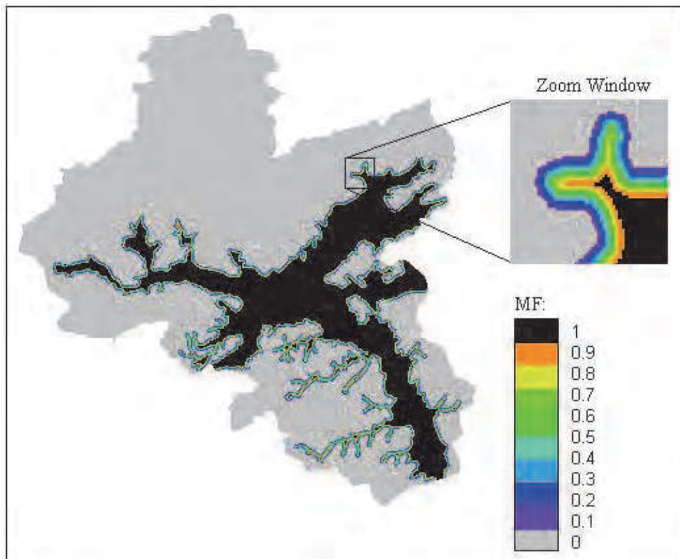
Fig. 6. Organic soil map with fuzzy boundaries
