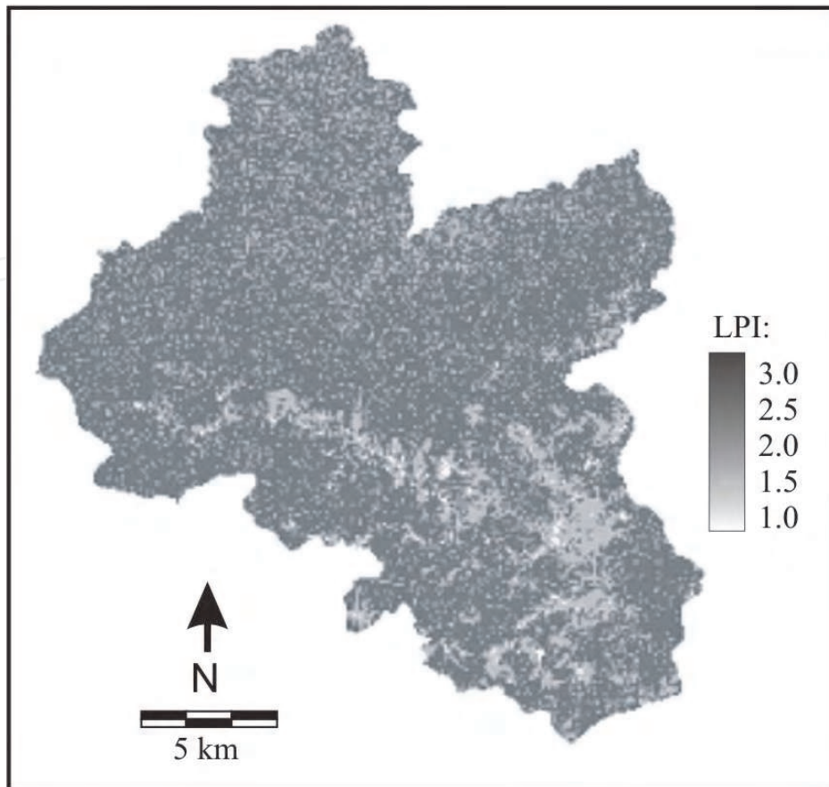
Fig. 2. Leaf Pigment Index (LPI) map
