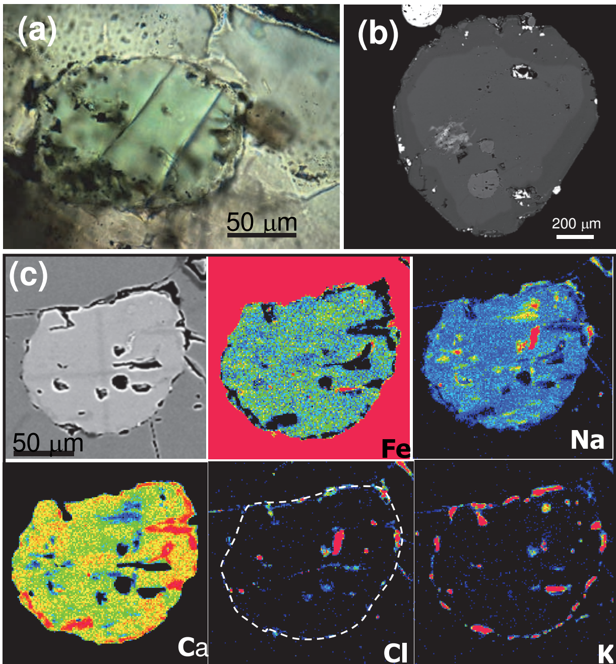
Fig. 9. A plane transmitted light photomicrograph (a) and back-scattered electron image (b) and X-ray element maps (c) of olivine-hosted clinopyroxene inclusions showing carbonate-chloride coatings and melt inclusions associated with clinopyroxene, and fine-scale compositional heterogeneity in terms of Fe, Ca and Na. Clinopyroxene on (c) is a larger inclusion on Fig. 9b. A contour of this inclusion is shown on the Cl K \alpha map by a dashed line.
