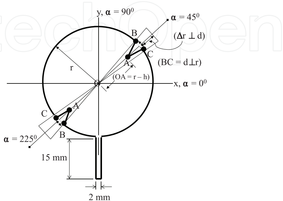
Fig. 3. Cellular energy harvesting antenna structure.
