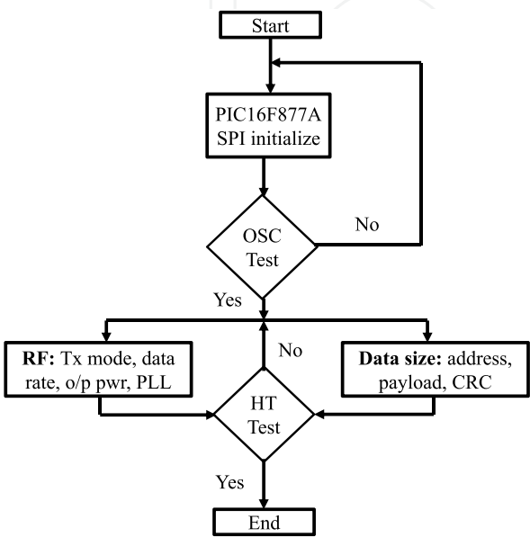
Fig. 27. Operation flow during transmission.
