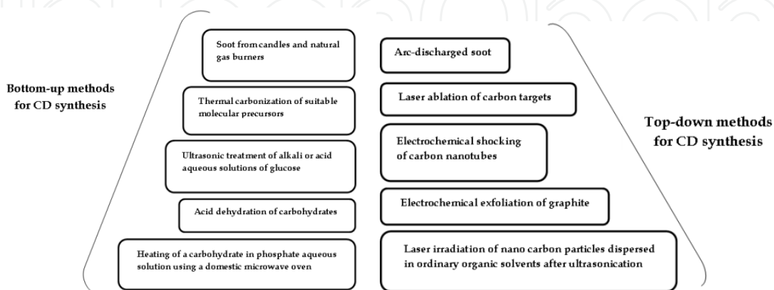
Fig. 1. Synthetic methodologies for CD.
