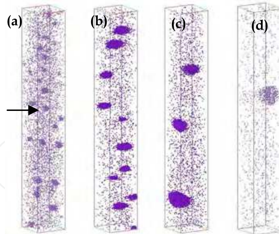
Fig. 20. Cu atomic mapping of Super304H aged for 1h(a), 100h(b), 500h(c) and 1,000h(d) at 650°C (size of selected box is 10nm×10nm×70nm)
