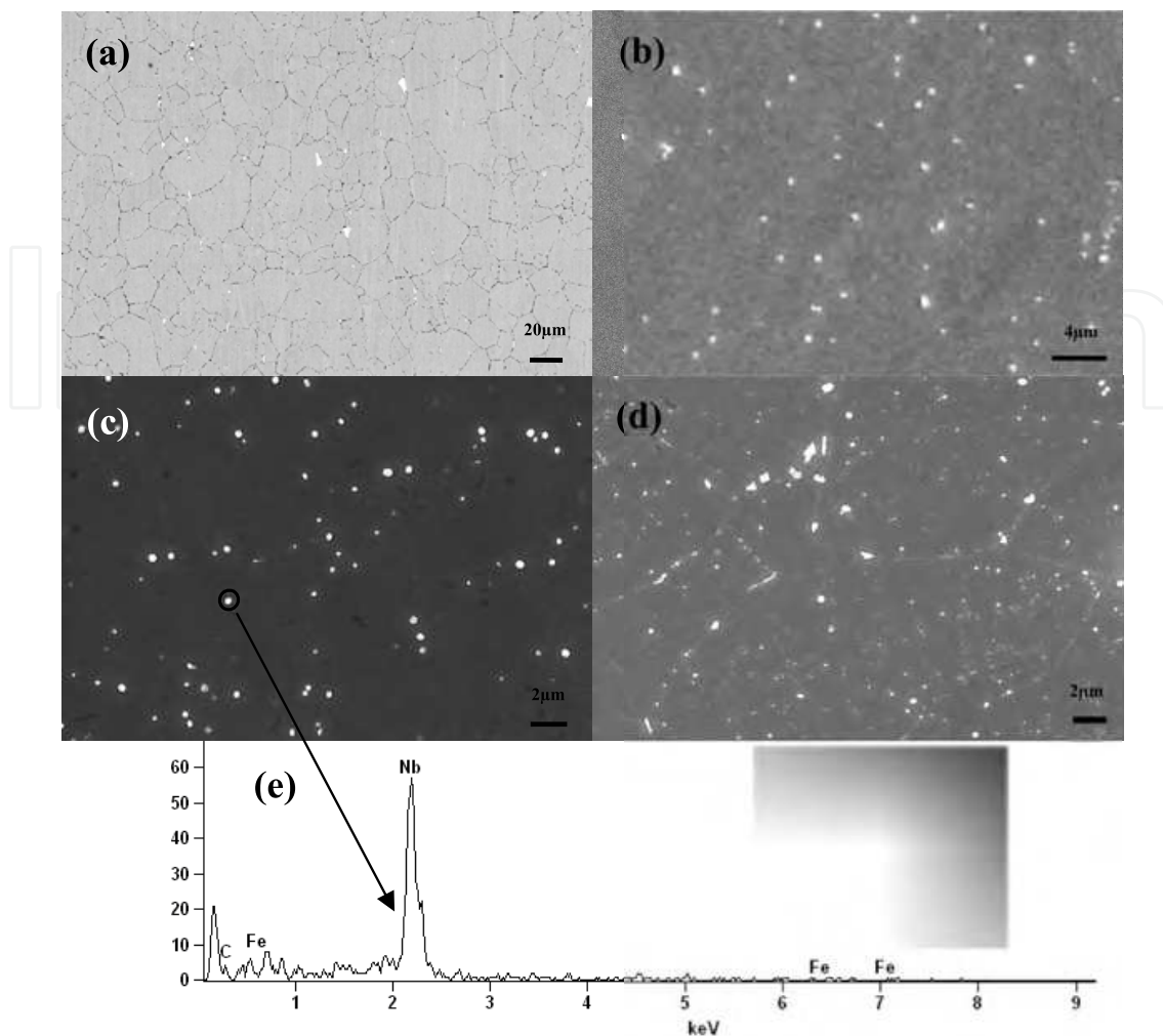
Fig. 6. SEM images of TP347H austenitic heat resistant steel after long-term aging at 650°C: solution treatment condition(a)(b), 650°C aging for 1,000h (c), 5,000h(d), and EDS spectrum corresponding to the precipitates in the grain(e)
