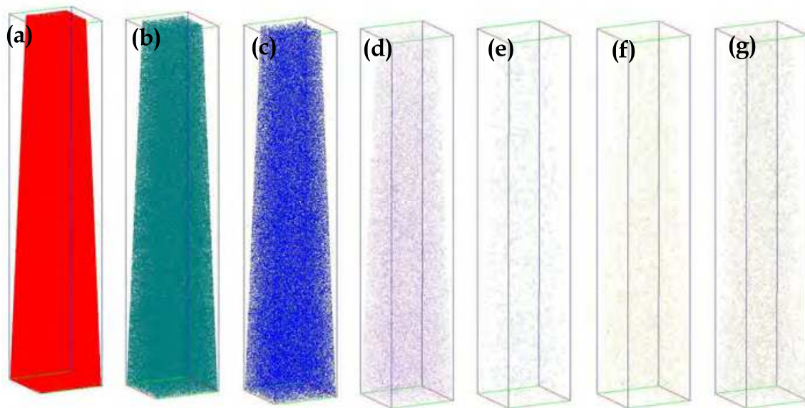
Fig. 19. Atomic mapping of the Super304H after solution treatment: Fe(a), Cr(b), Ni(c), Cu(d), Nb(e), C(f) and N(g) (size of selected box is 10nm×10nm×70nm)
