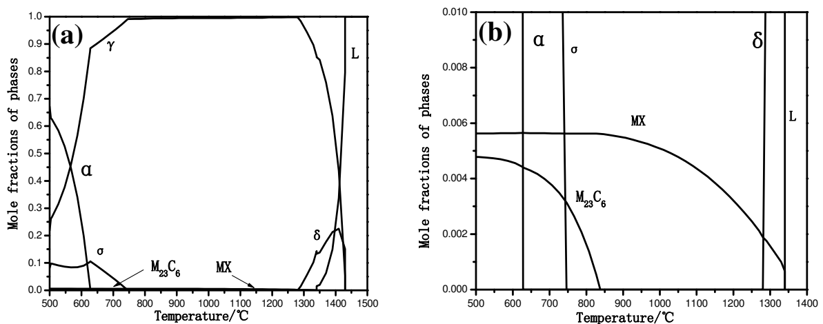
Fig. 10. Calculated mole fractions of phases on temperatures in TP347H steel (a) and its partial magnified diagram (b)
