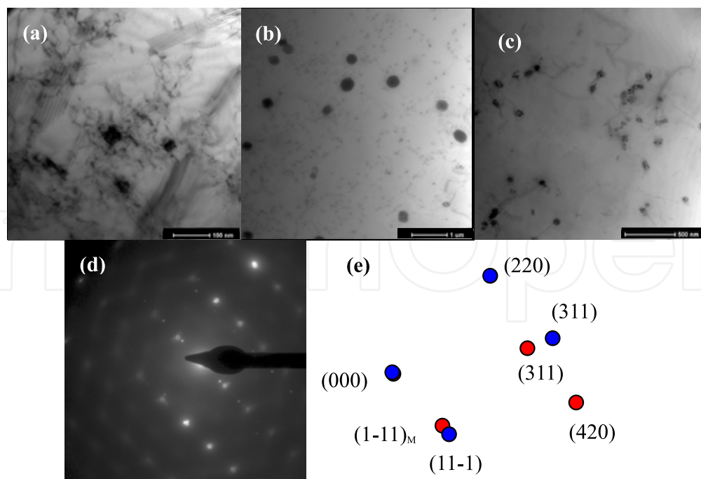
Fig. 9. TEM images and diffraction patterns of precipitations in TP347H steel after long-term aging at 650°C (a) 5,000h; (b) and (c) 10,000h; (d) and (e) diffraction patterns of \gamma -matrix and precipitation in(c)
