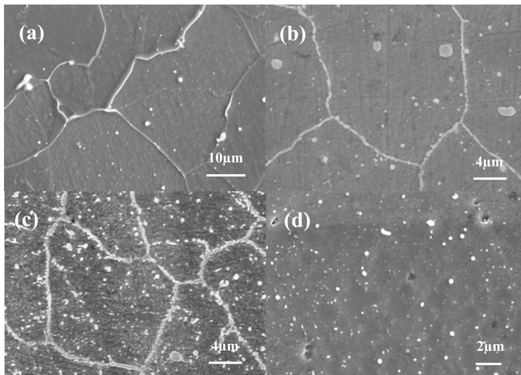
Fig. 16. SEM images of Super304H after solid solution treatment(a), aging at 650°C for different times 500h(b), 5,000h(c) and high magnified image in grain aging for 10,000h(d)
