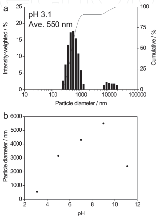
Fig. 19. (a): Particle size distribution of anatase \text{TiO}_2 particles at pH 3.1. (b): Particle size of anatase \text{TiO}_2 particles as a function of pH. Reprinted with permission from Ref. 77 , Masuda, Y. and Kato, K., 2008, Cryst. Growth Des. , 8, 3213. Copyright @American Chemical Society
