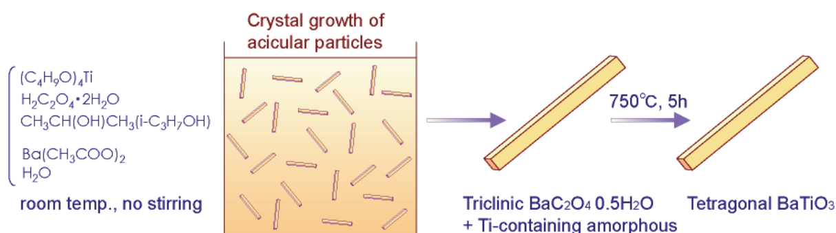
Fig. 1. Conceptual process for fabricating acicular \text{BaTiO}_3 particles. Morphology control of \text{BaC}_2\text{O}_4 \cdot 0.5\text{H}_2\text{O} particles and phase transition to \text{BaTiO}_3 . Reprinted with permission from Ref.1, Masuda, Y., Yamada, T. and Koumoto, K., 2008, Cryst. Growth Des. , 8, 169. Copyright ©American Chemical Society
