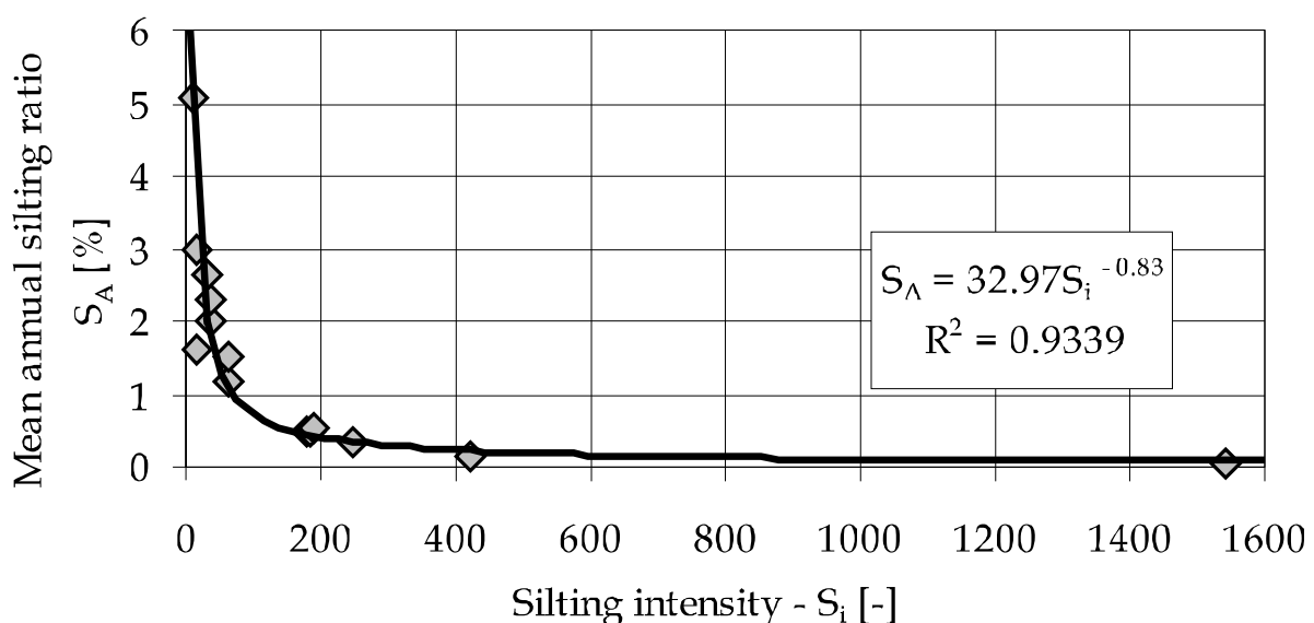
Fig. 2. Regression dependence of the mean annual silting ratio ( S_A ) defined on the basis of measurements and silting intensity ( S_i ) according to the Šamov's equation
