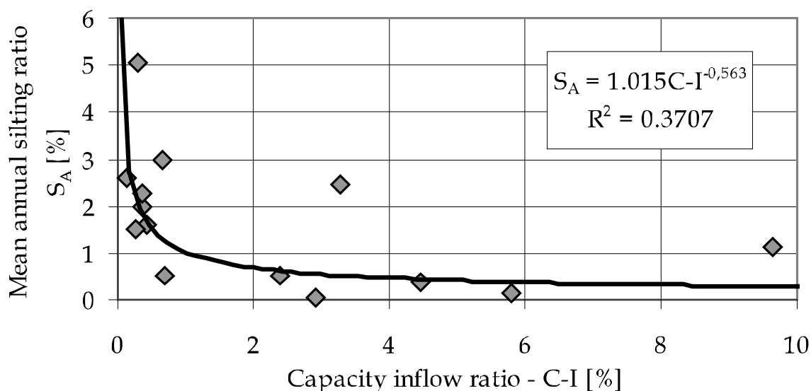
Fig. 3. Regression dependence of the mean annual silting ratio ( S_A ) defined on the basis of measurements and capacity-inflow ratio (C-I)
