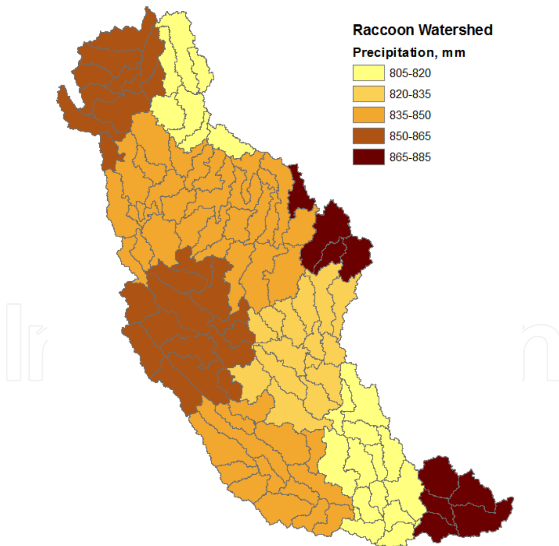
Fig. 5. Spatial representation of precipitation on a long-term annual basis
