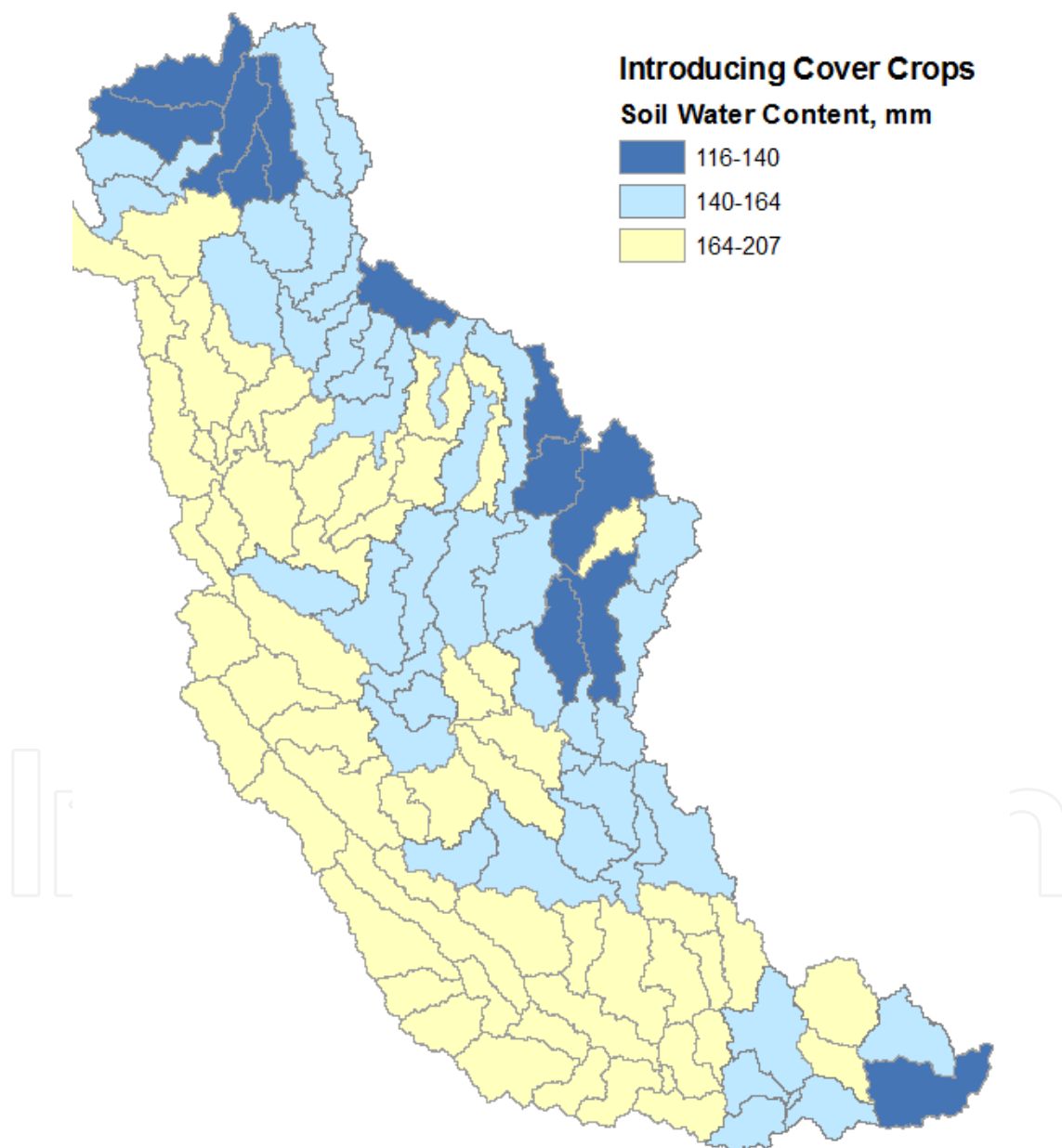
Fig. 9. Soil moisture content (after introducing winter cover crop) as predicted by SWAT at subwatershed scale on a long-term basis
