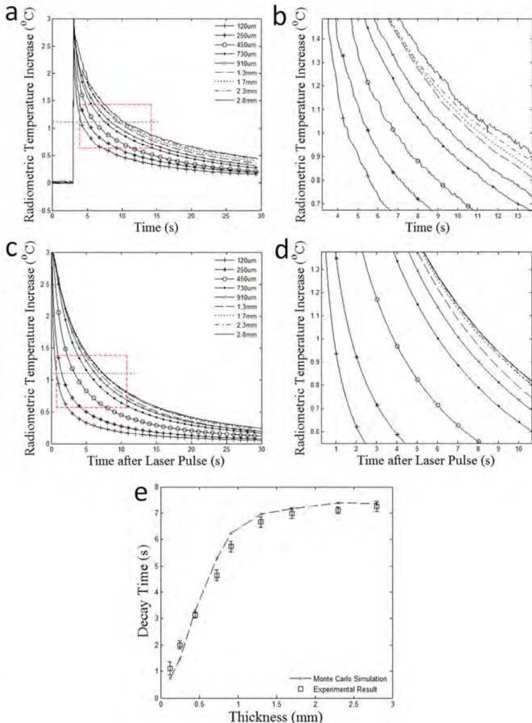
Fig. 9. (a) Measured radiometric temperature increase from PDMS tissue phantoms (top-layer is 120 \mu\text{m} -2.8 mm thick respectively - mimicking different CMM thicknesses). (b) Measured radiometric temperature increase in the window indicated in (a). (c) Simulated radiometric temperature increase. (d) Simulated radiometric temperature increase in the window indicated in (c). The dashed lines in (a,c) indicate when peak radiometric temperature increase decays to 37% of the maximum. (e) Decay time of the PDMS tissue phantoms with different top-layer thicknesses from experiment (square box) and simulation (dashed line). Image adopted from T. Wang et al., 2011.
